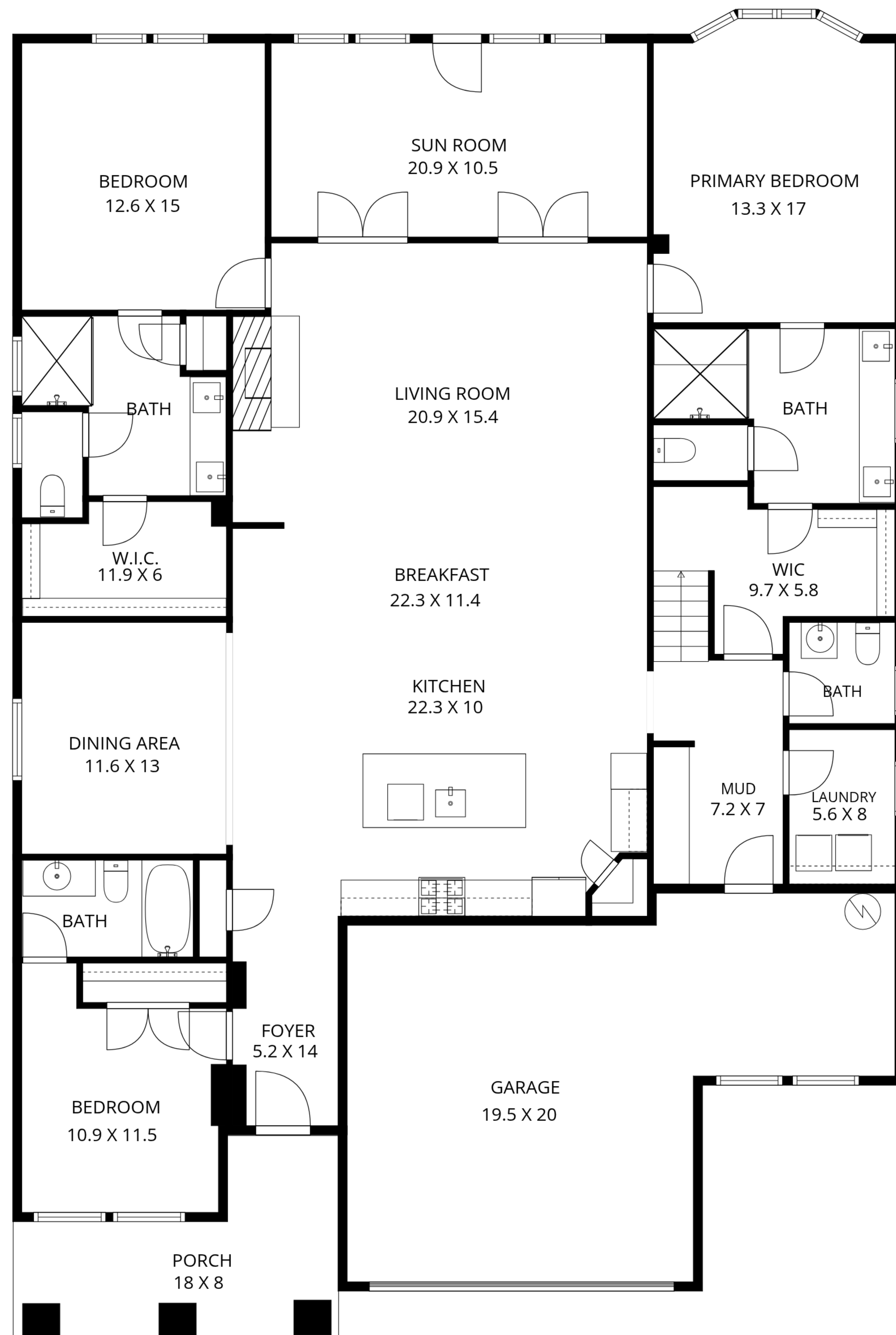
1ST FLOOR
