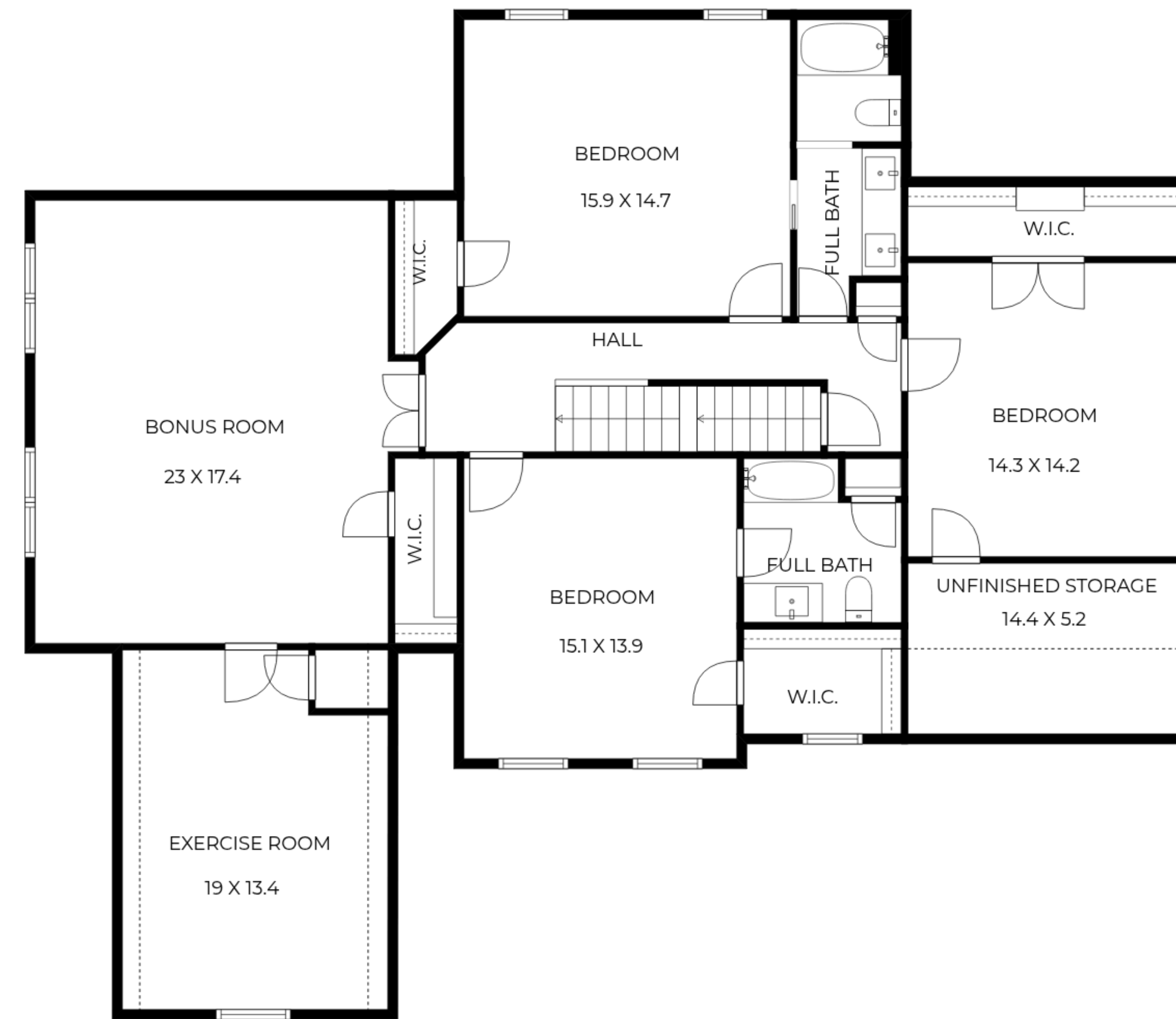
2ND FLOOR
