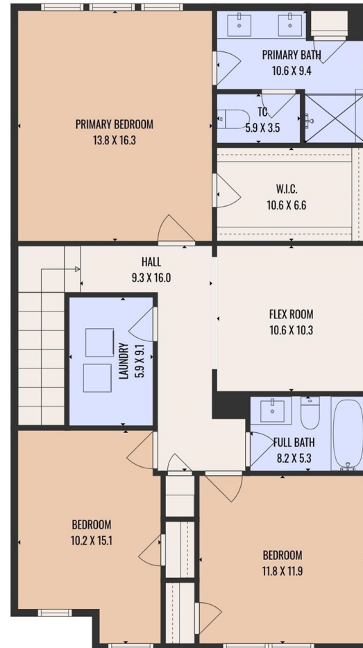
2ND FLOOR
