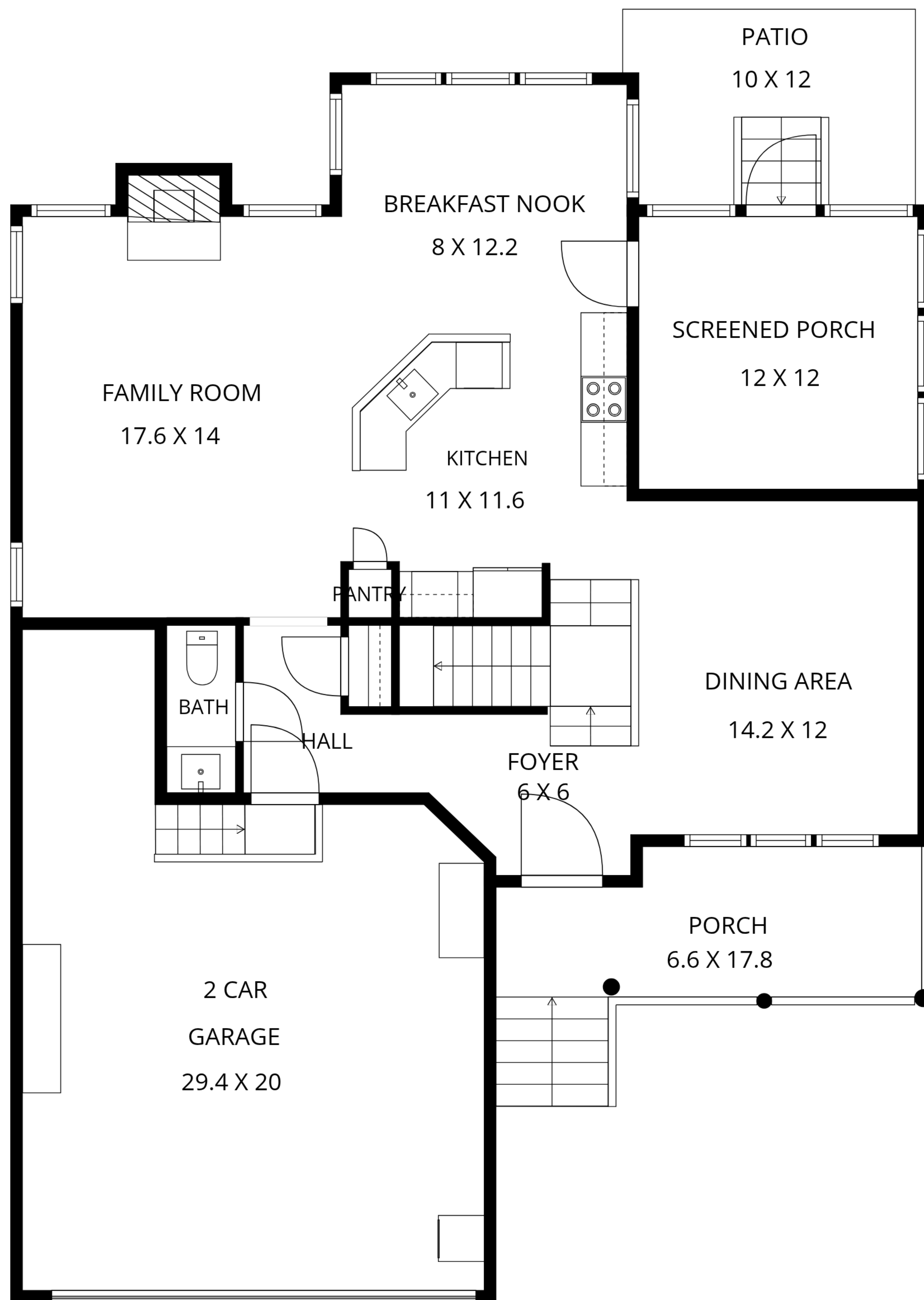
1ST FLOOR
