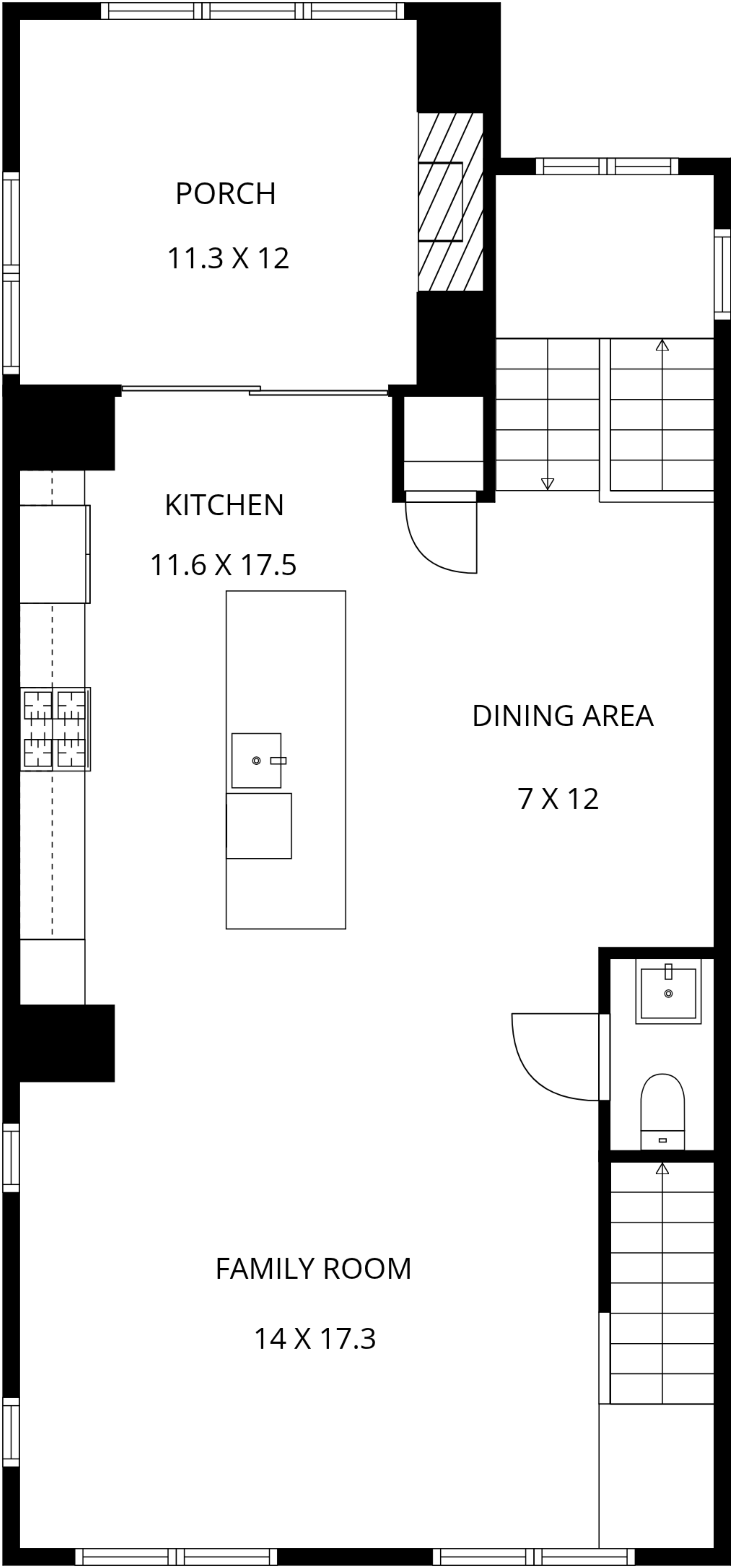
2ND FLOOR
