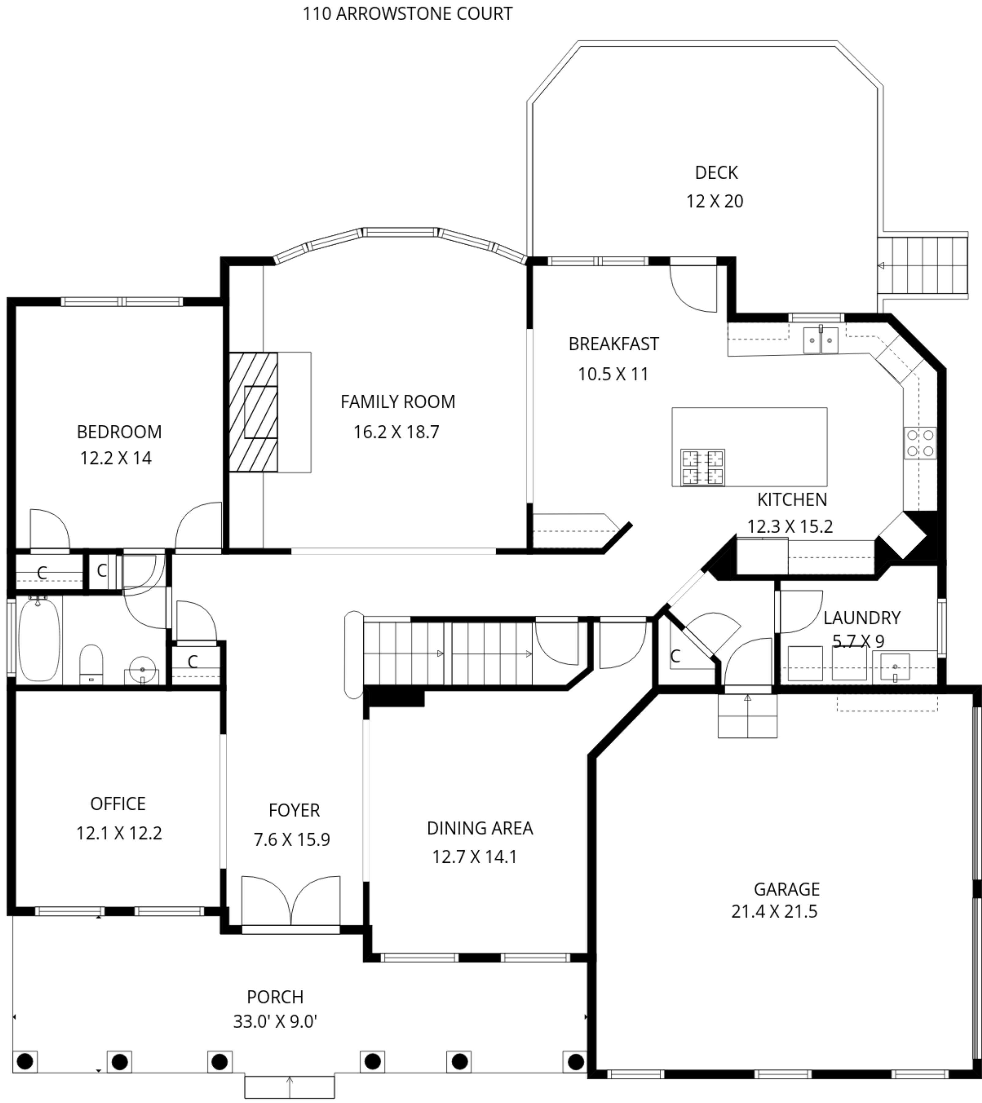
1ST FLOOR
