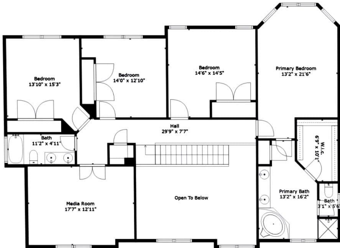
Floor 2
