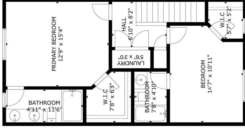
FLOOR 2
