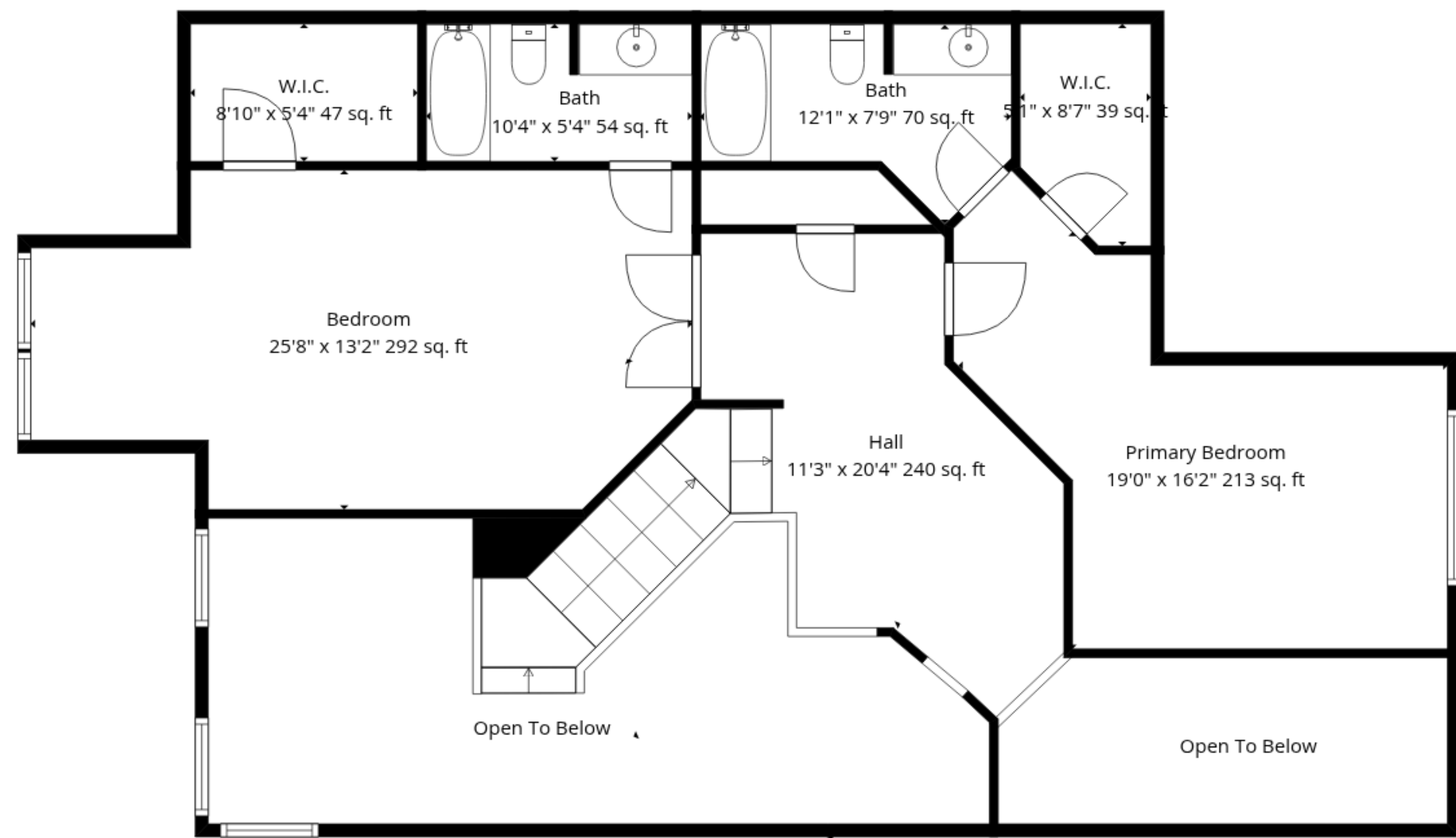
2nd Floor
