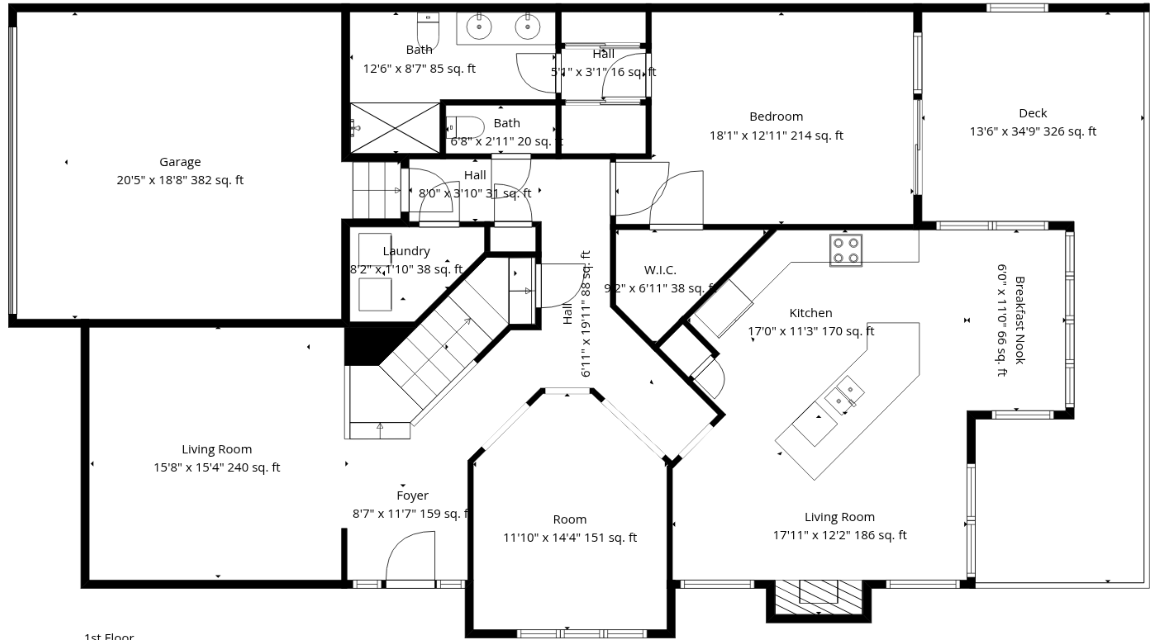
1st Floor
