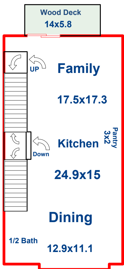
Second Floor
