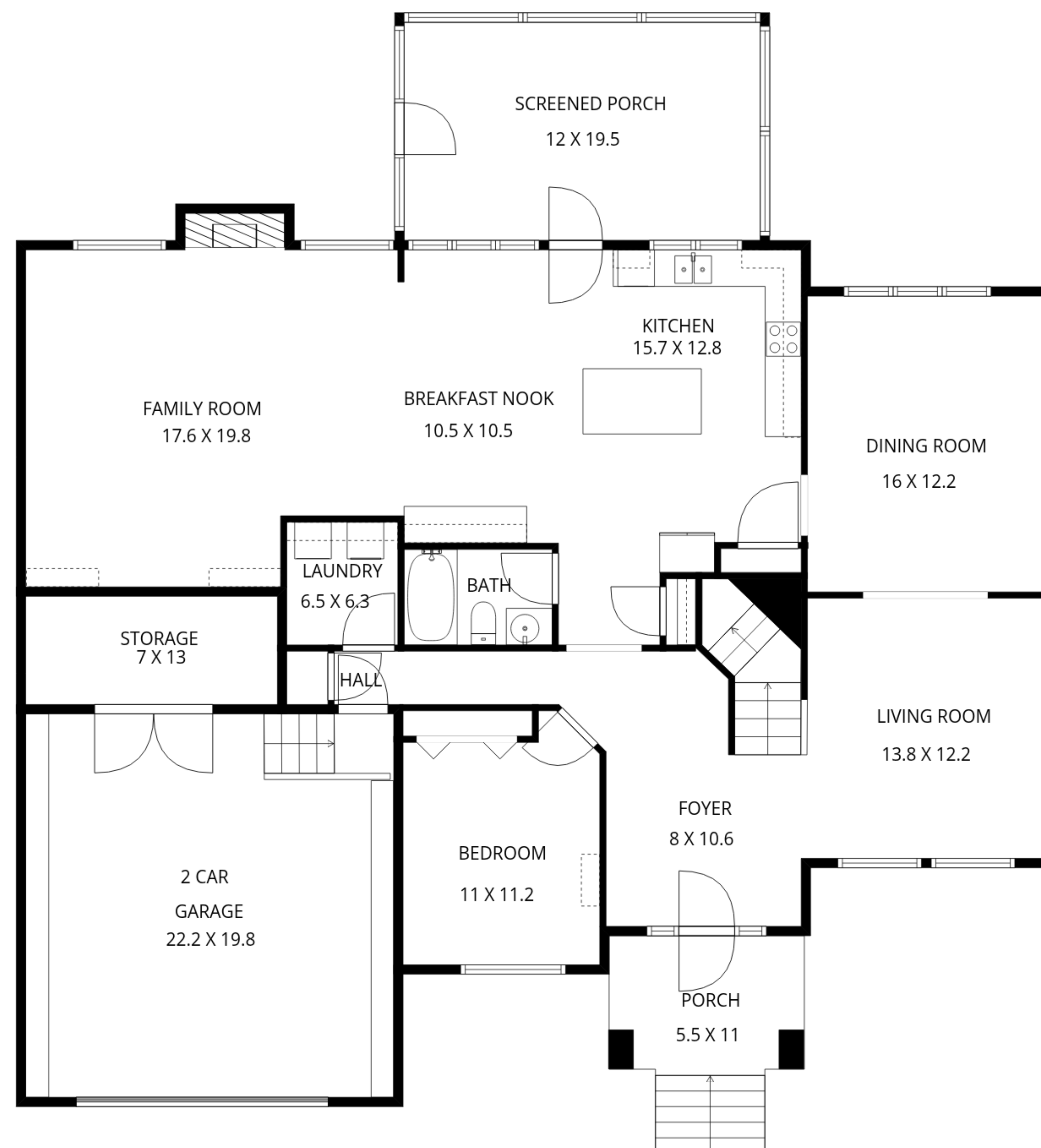
1ST FLOOR
