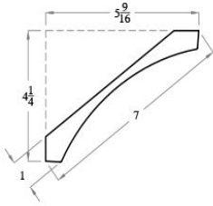
EC81 CROWN ROUND SHOE MOULDING SIMPLE CASING
