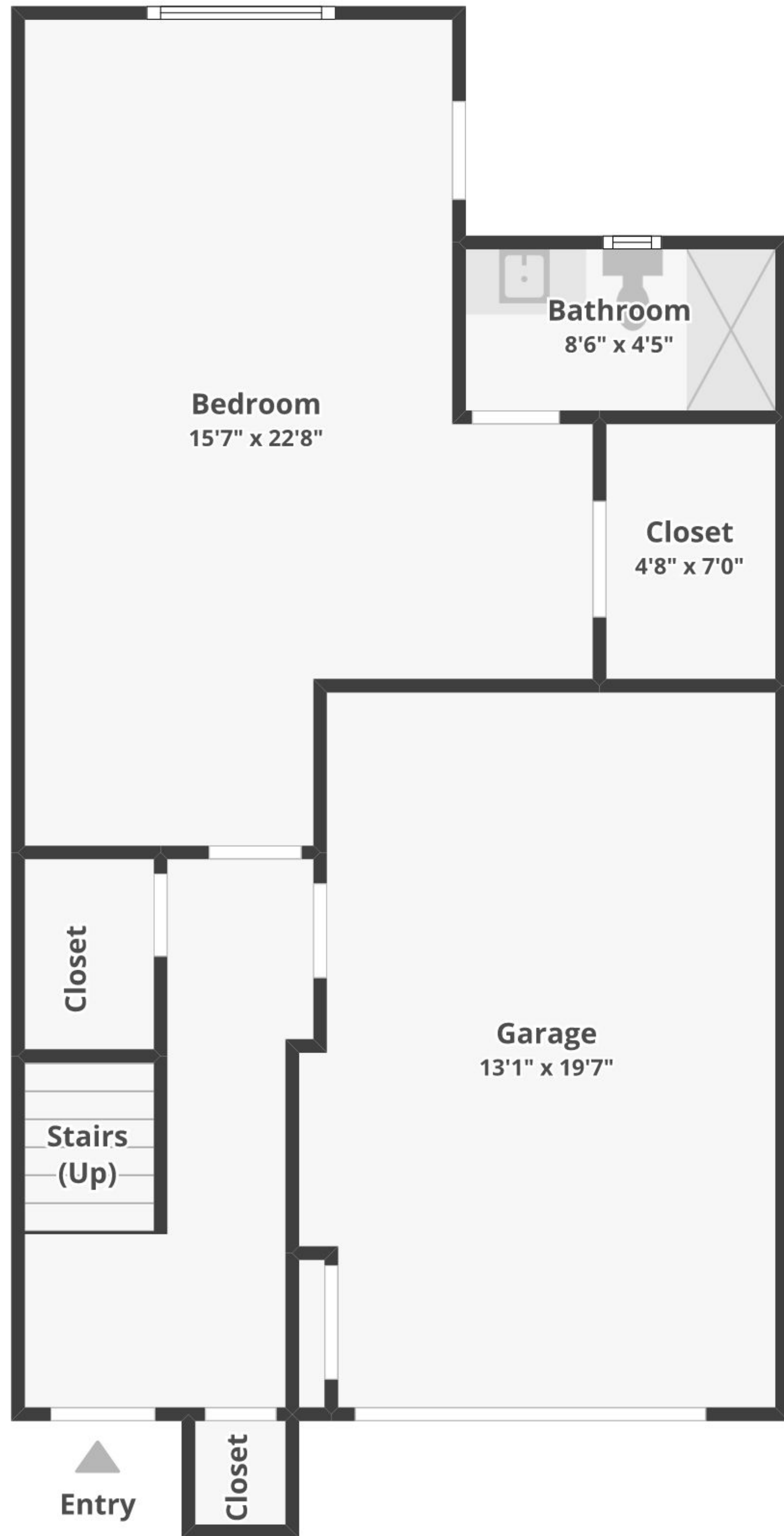
FLOOR 1
