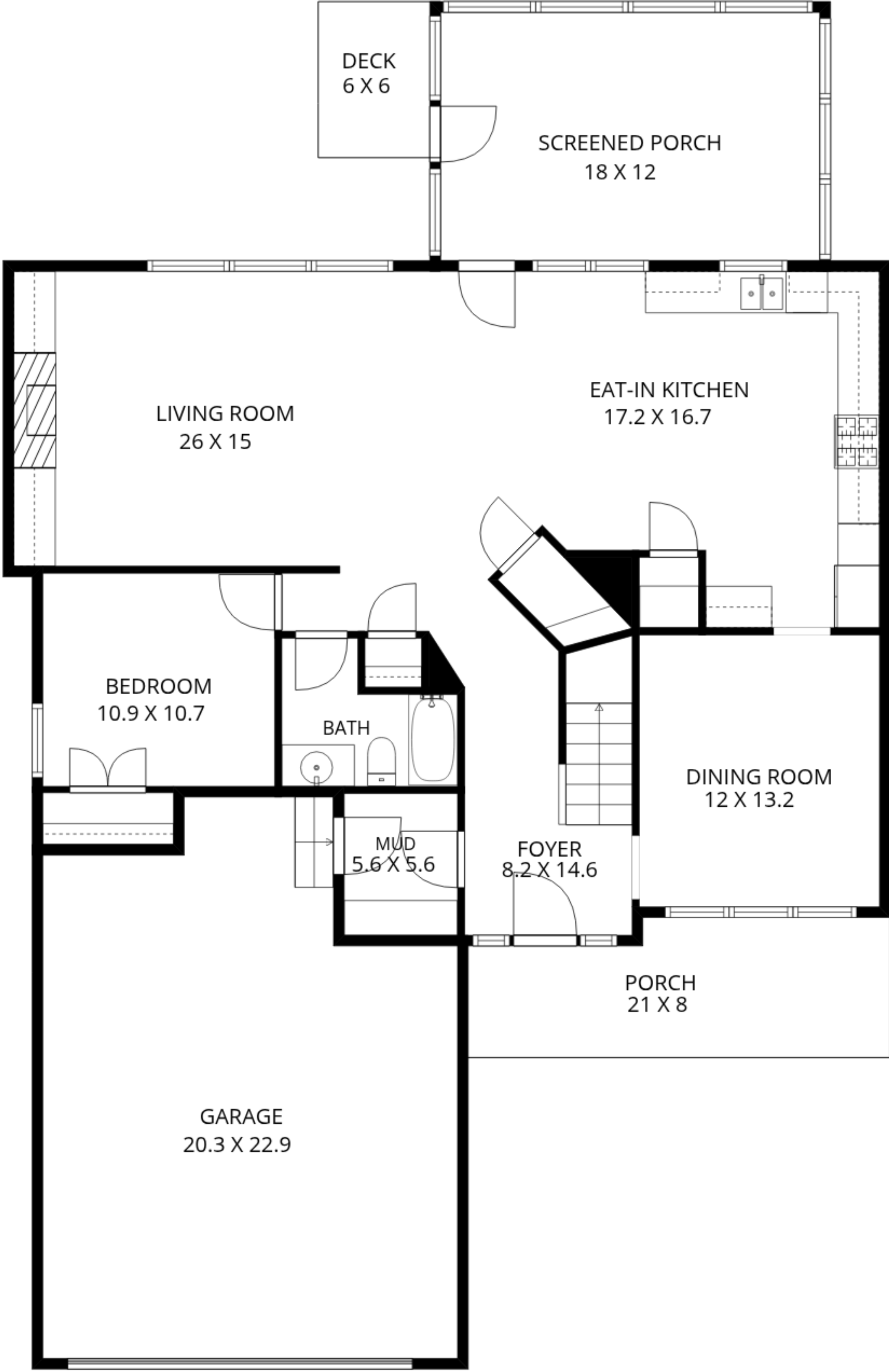
1ST FLOOR
