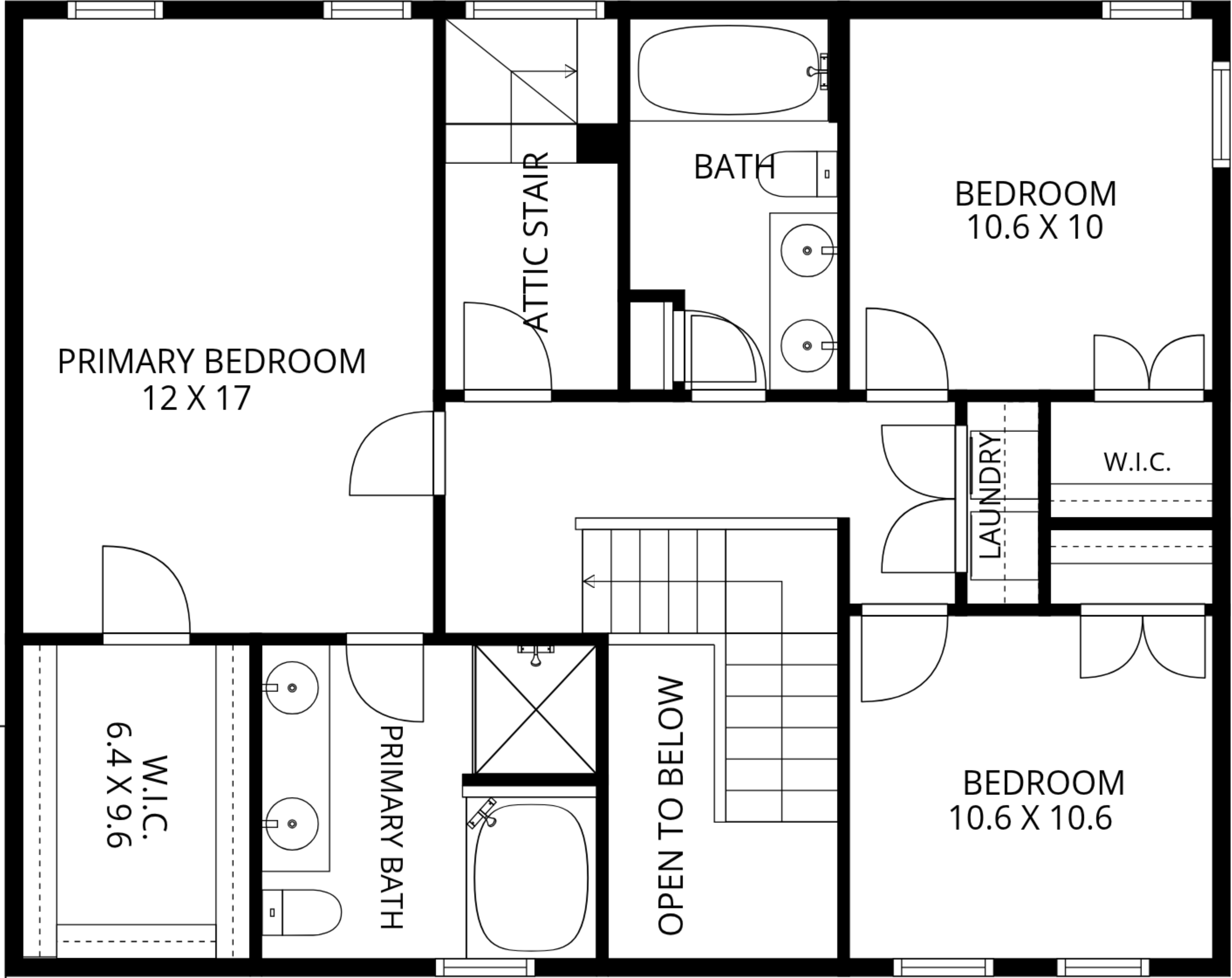
2ND FLOOR
