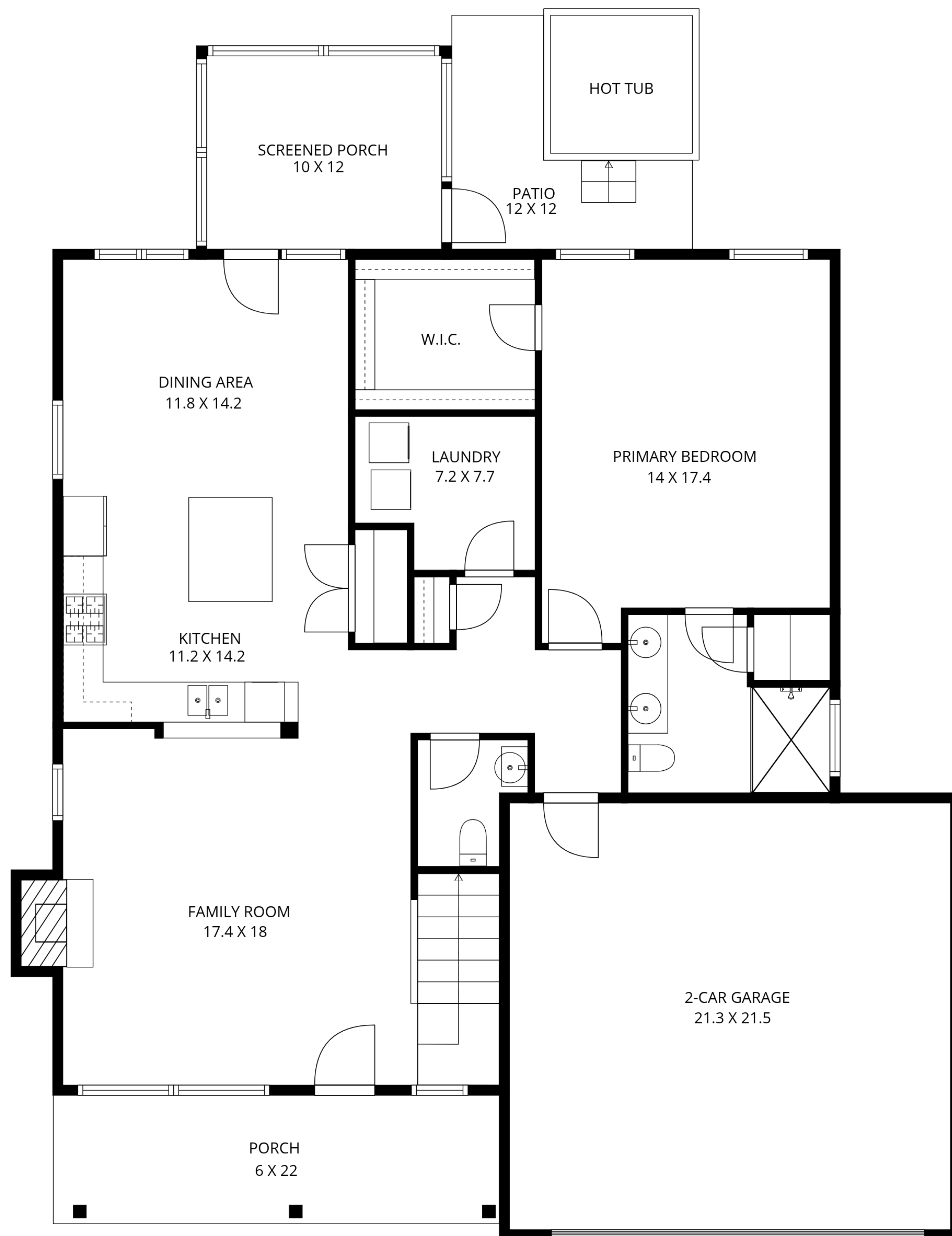
1ST FLOOR
