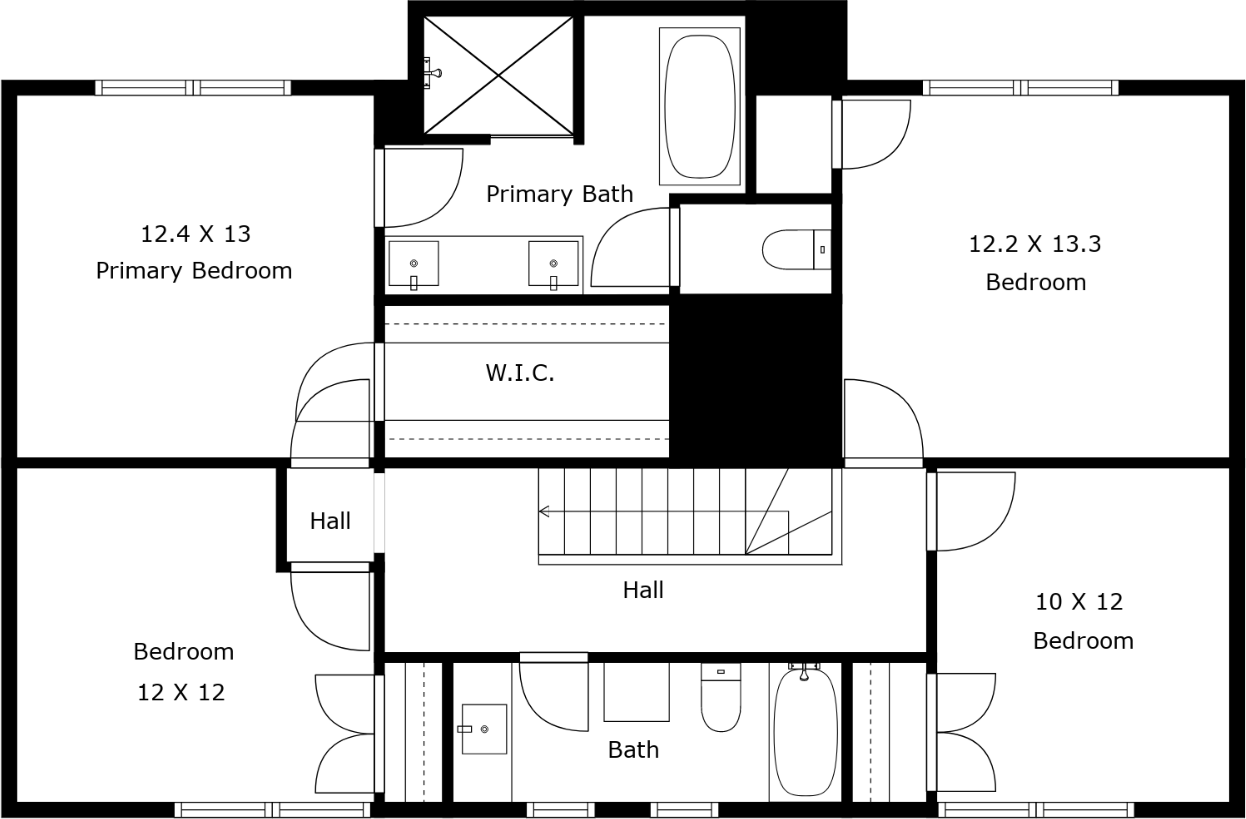
Floor 2
