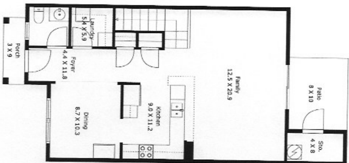
Floor 1
