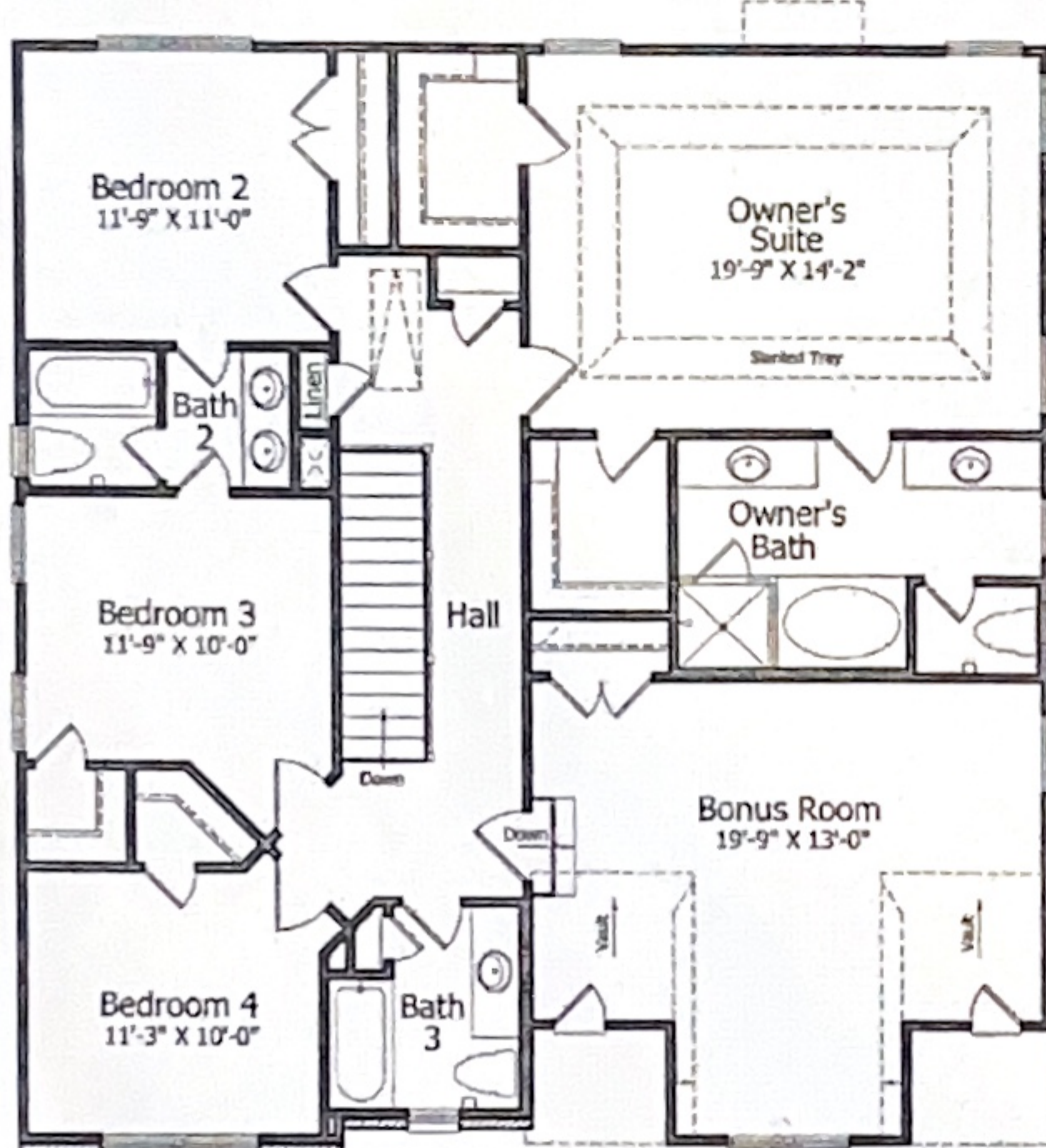
Second Floor
