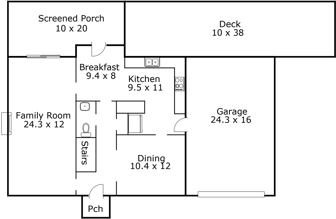
First Floor
