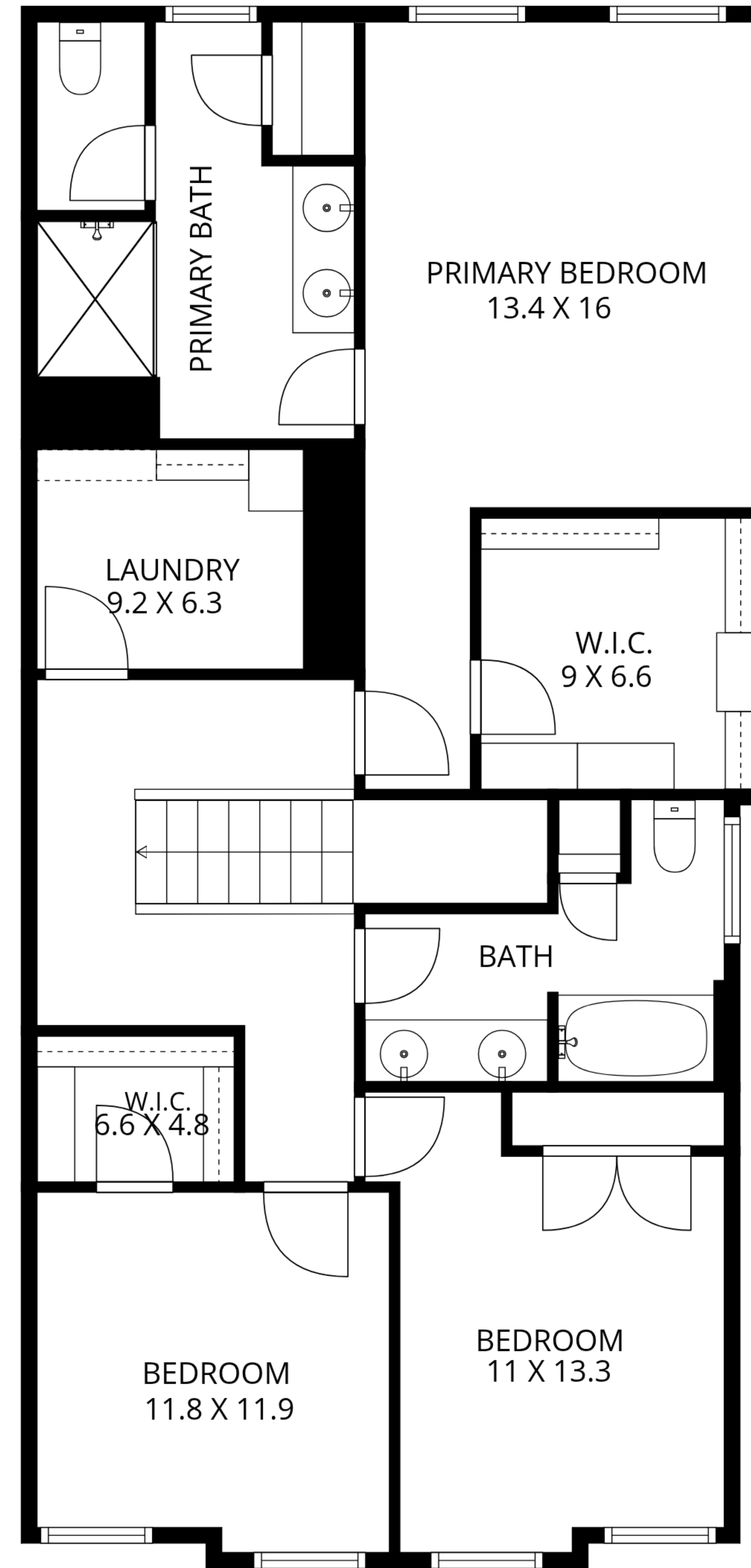
2ND FLOOR
