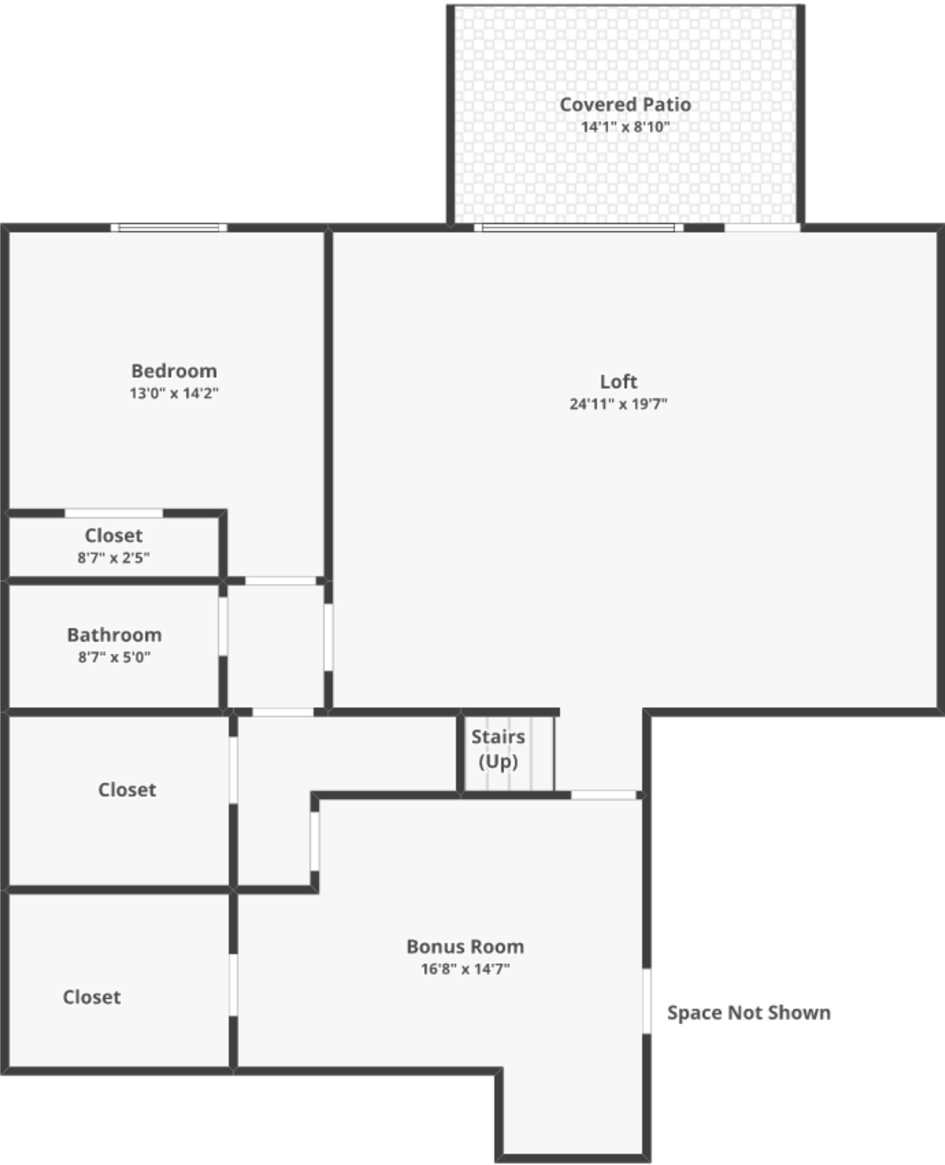
BASEMENT
