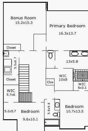
2nd Floor
