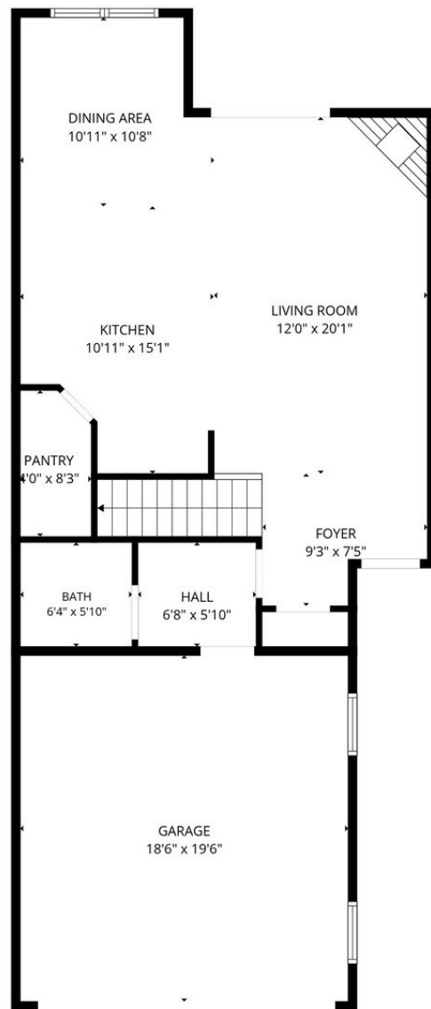
1st floor
