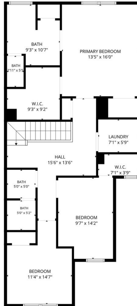
2nd floor
