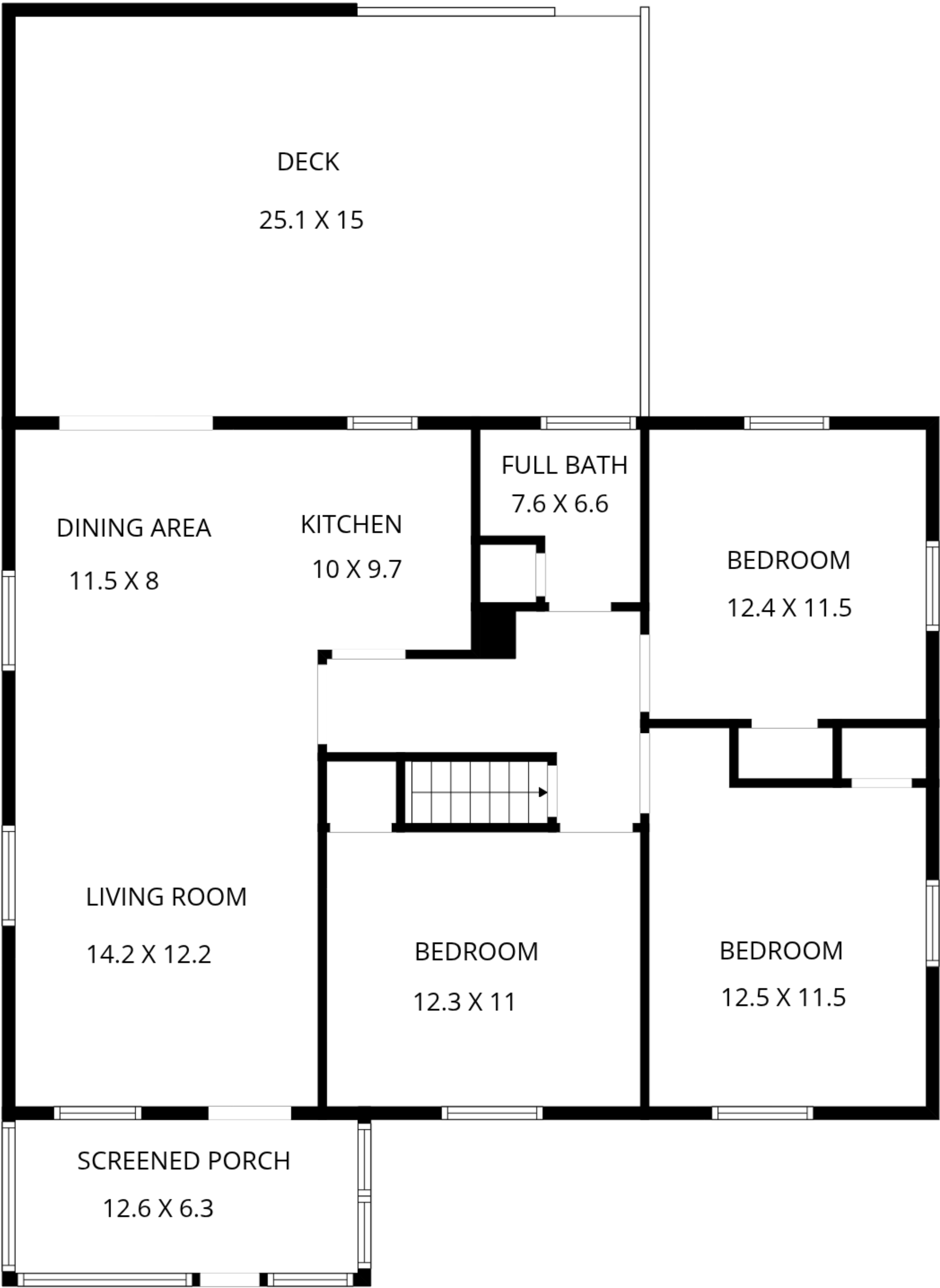
1st floor
