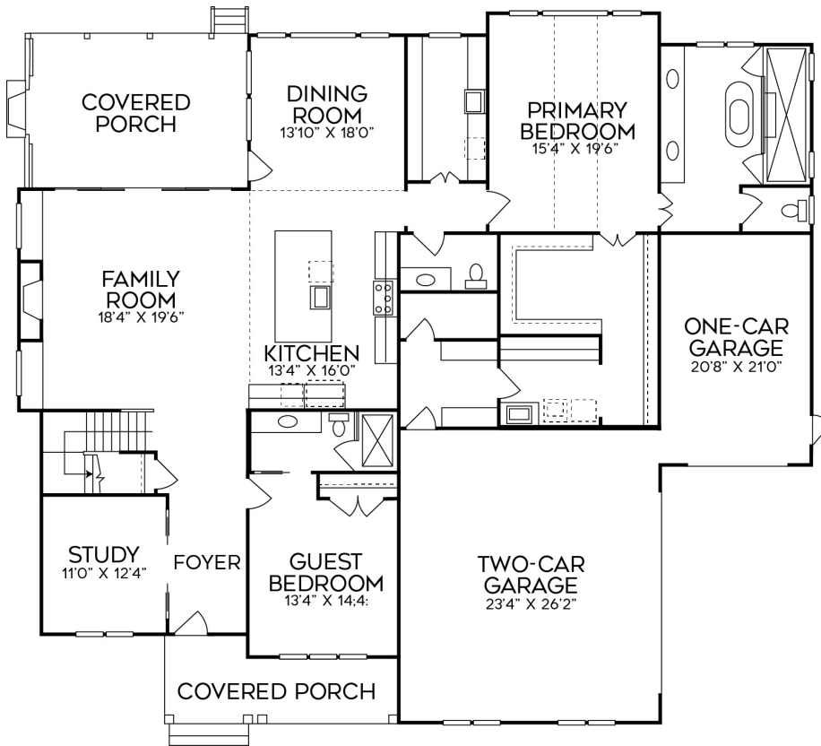
FIRST FLOOR
