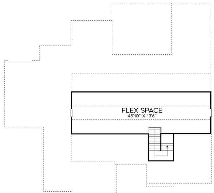
Third Floor
