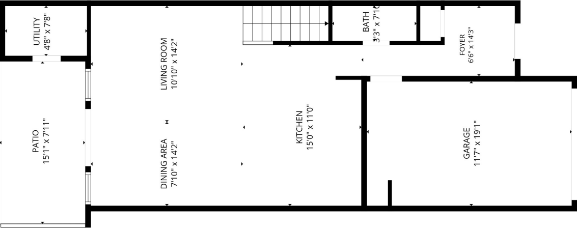
1st floor
