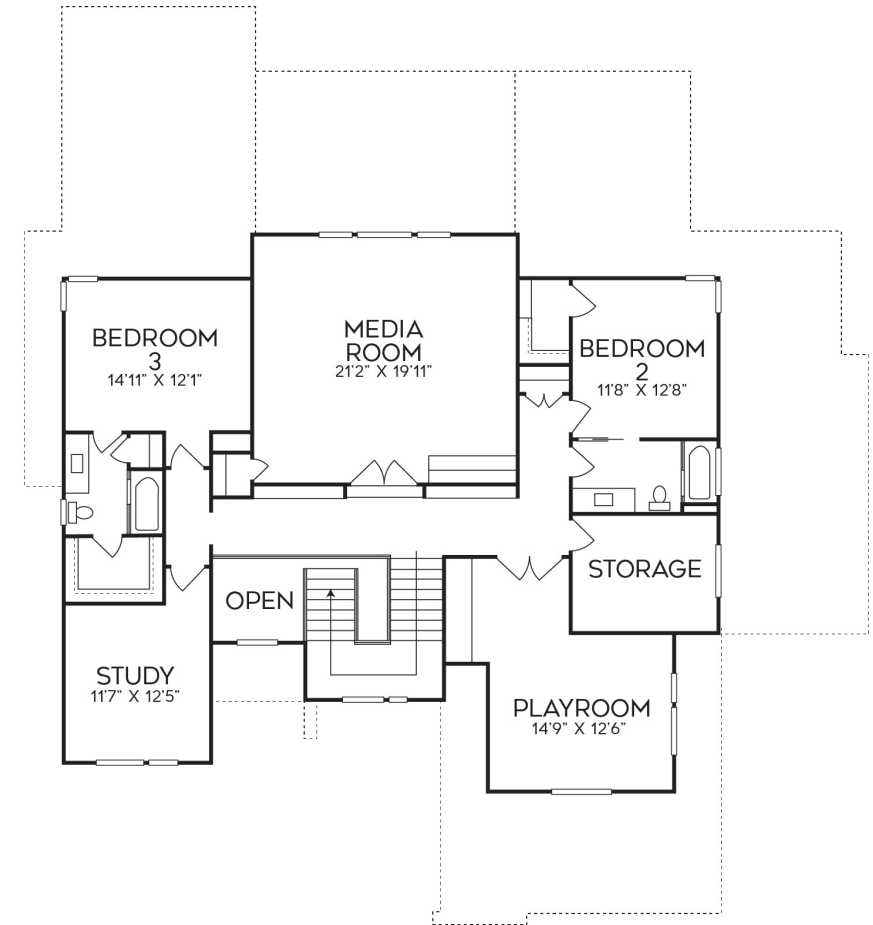
SECOND FLOOR
