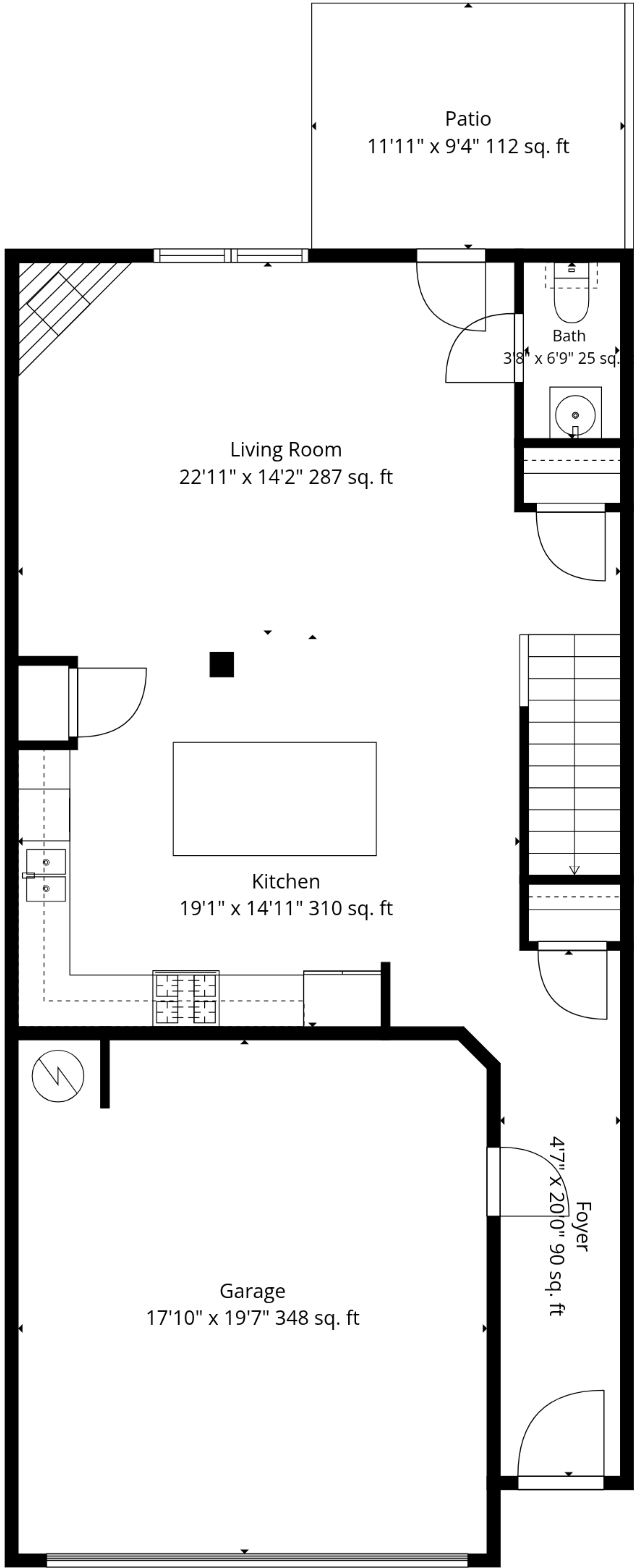
1st Floor
