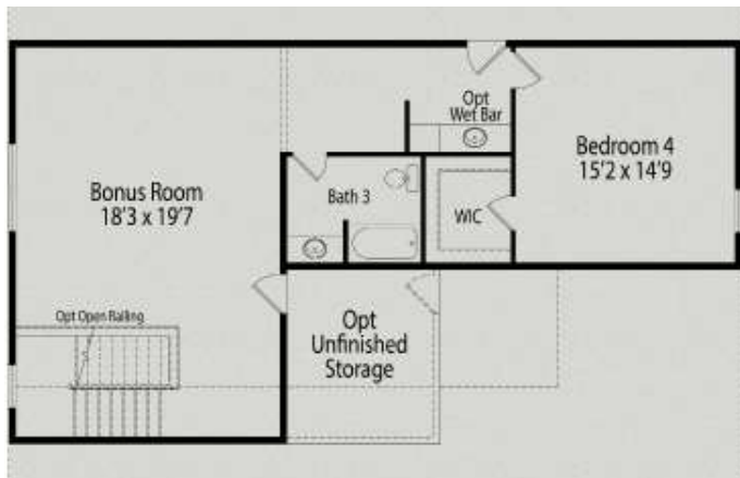
OPTIONAL BONUS ROOM WITH BEDROOM 4
