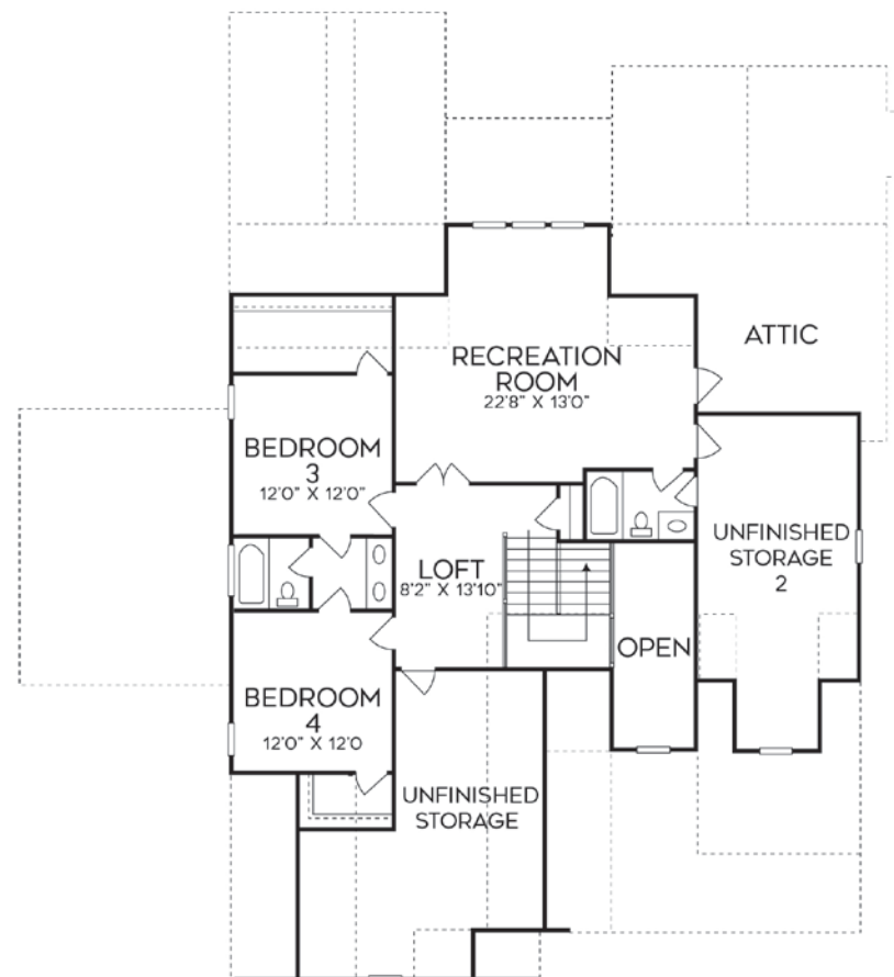
SECOND FLOOR
