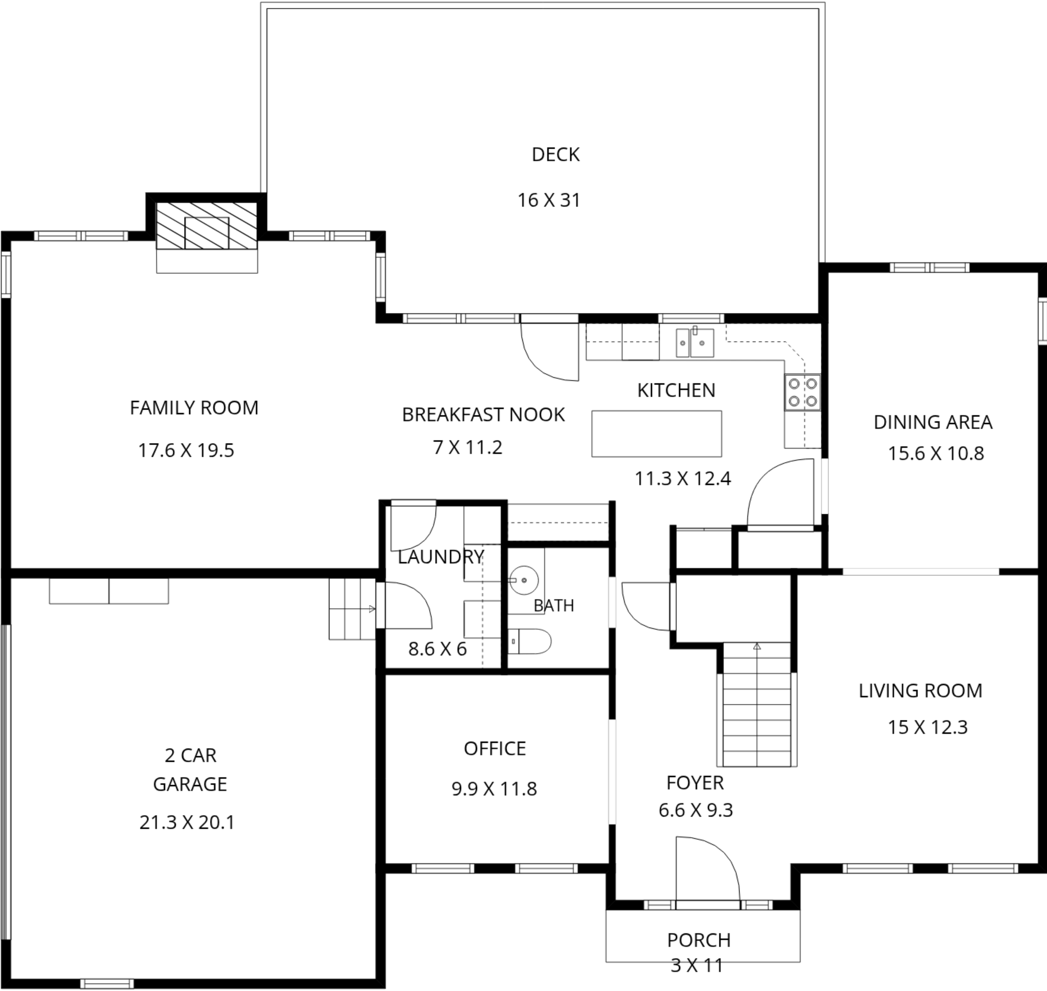
1ST FLOOR
