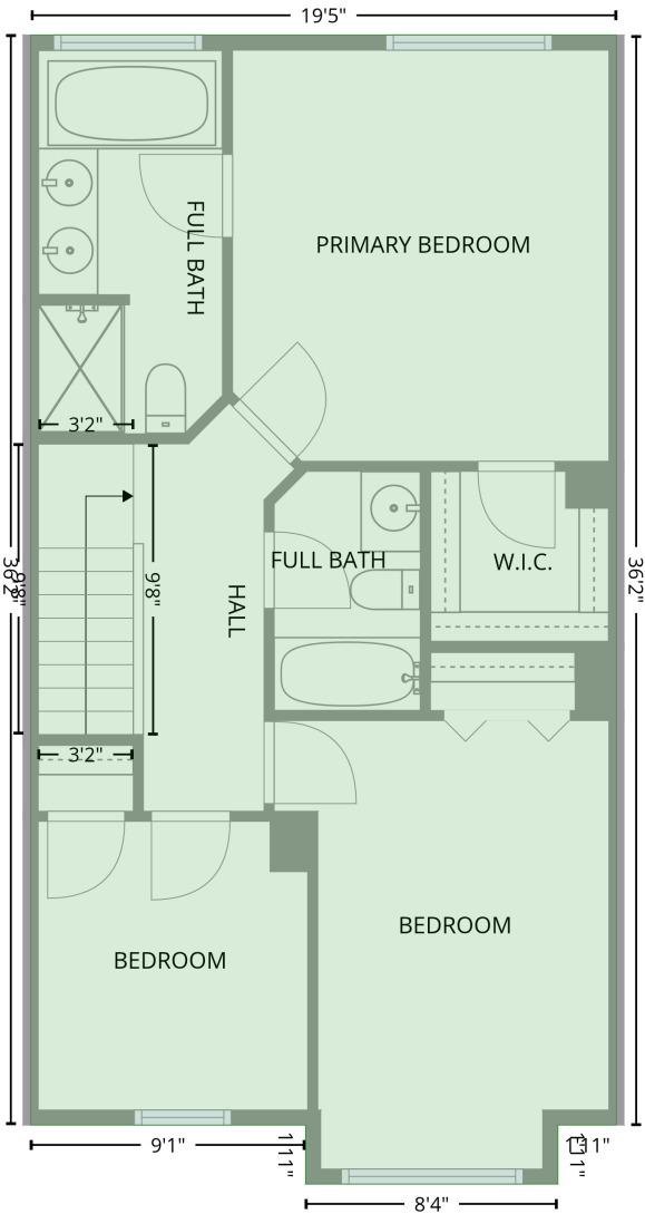
2nd floor [AREA: 719]
