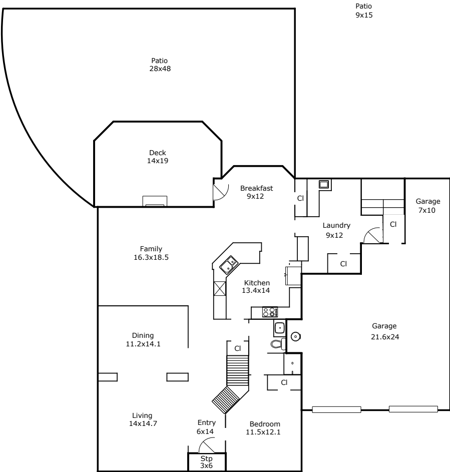
First Floor
