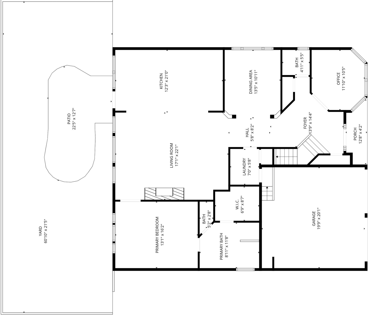
1st floor
