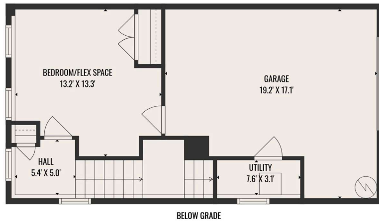
BASEMENT (FINISHED)
