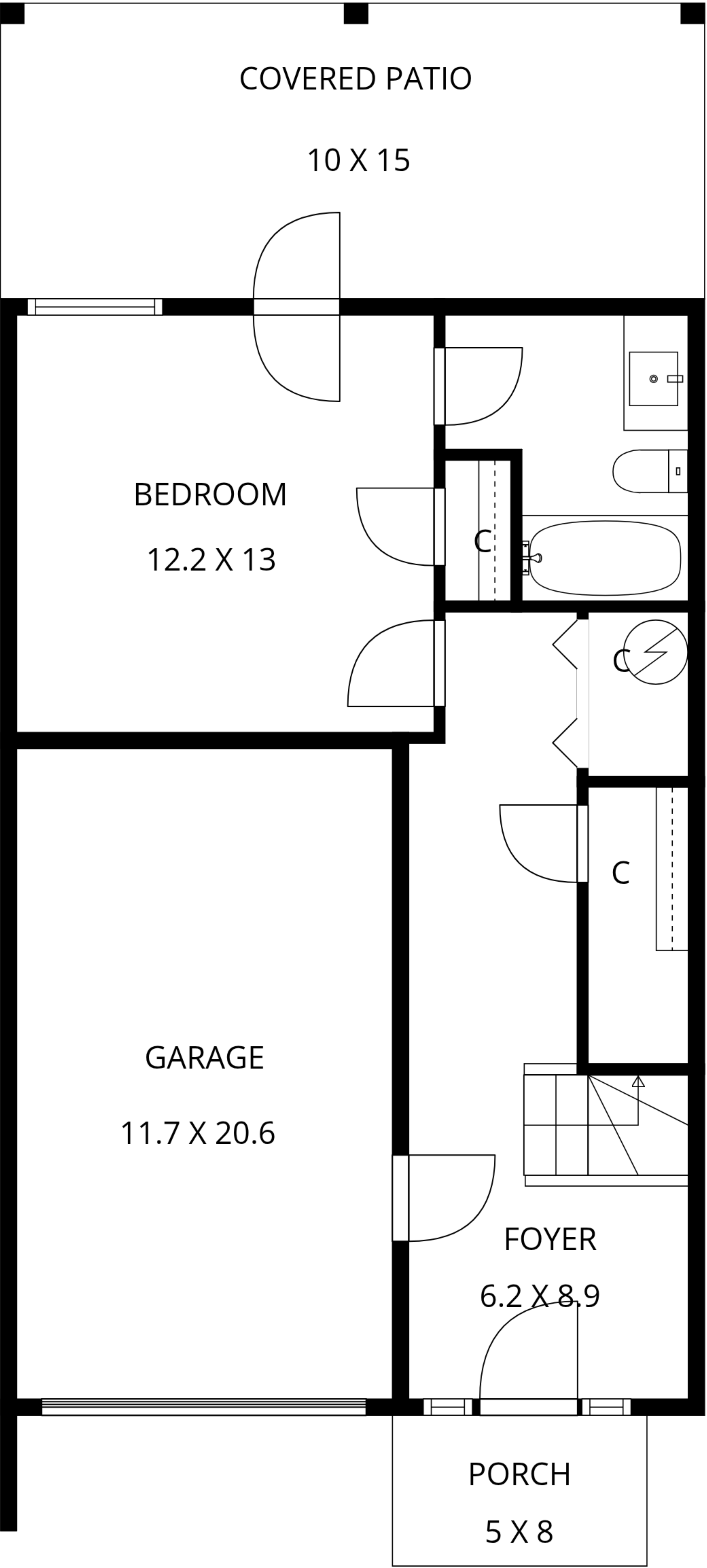
1ST FLOOR
