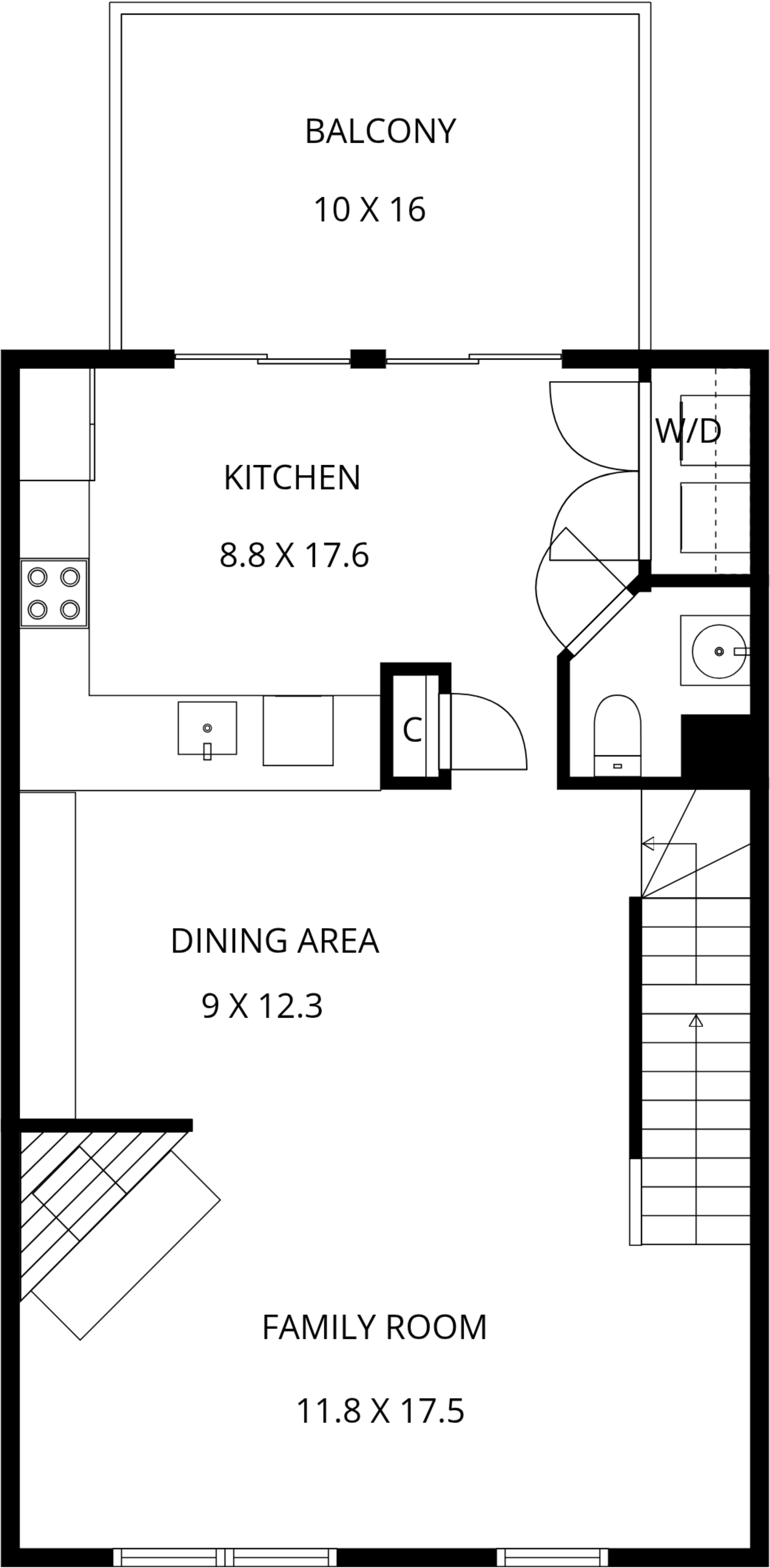
2ND FLOOR
