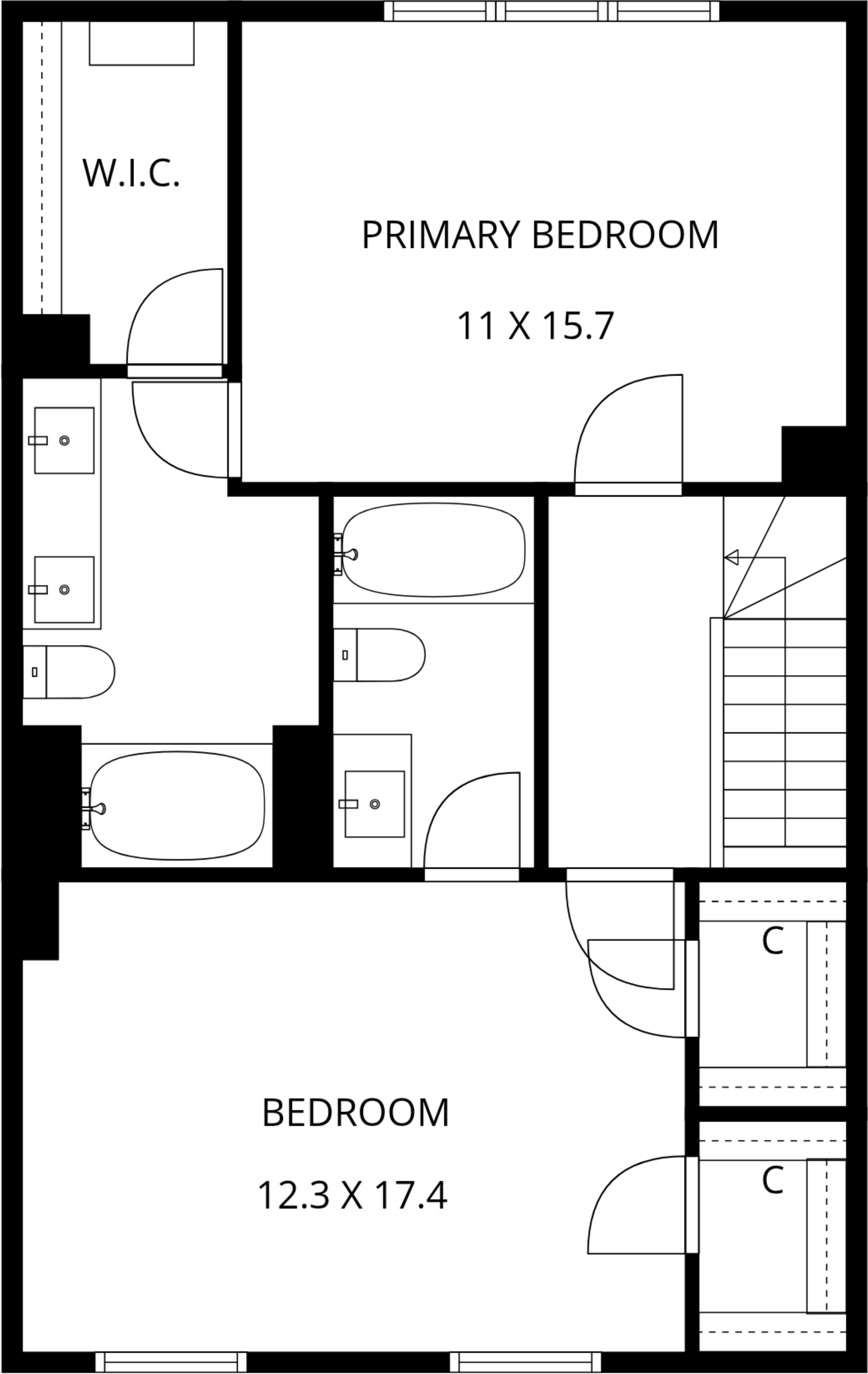
3RD FLOOR
