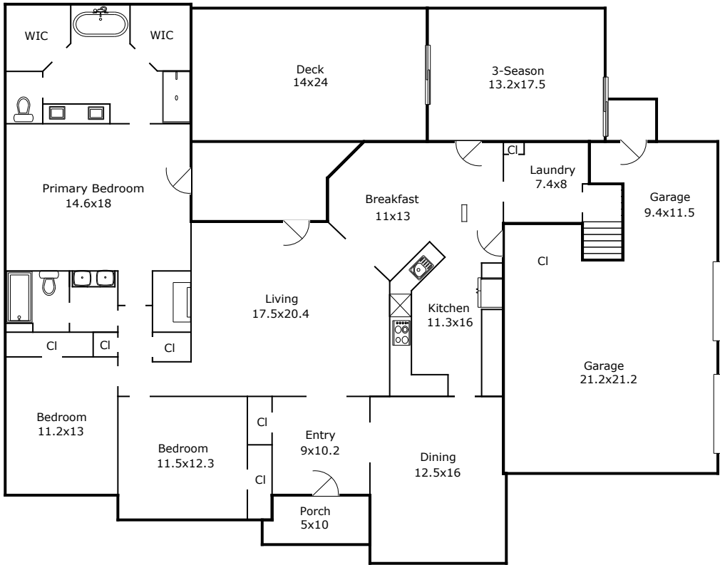
First Floor
