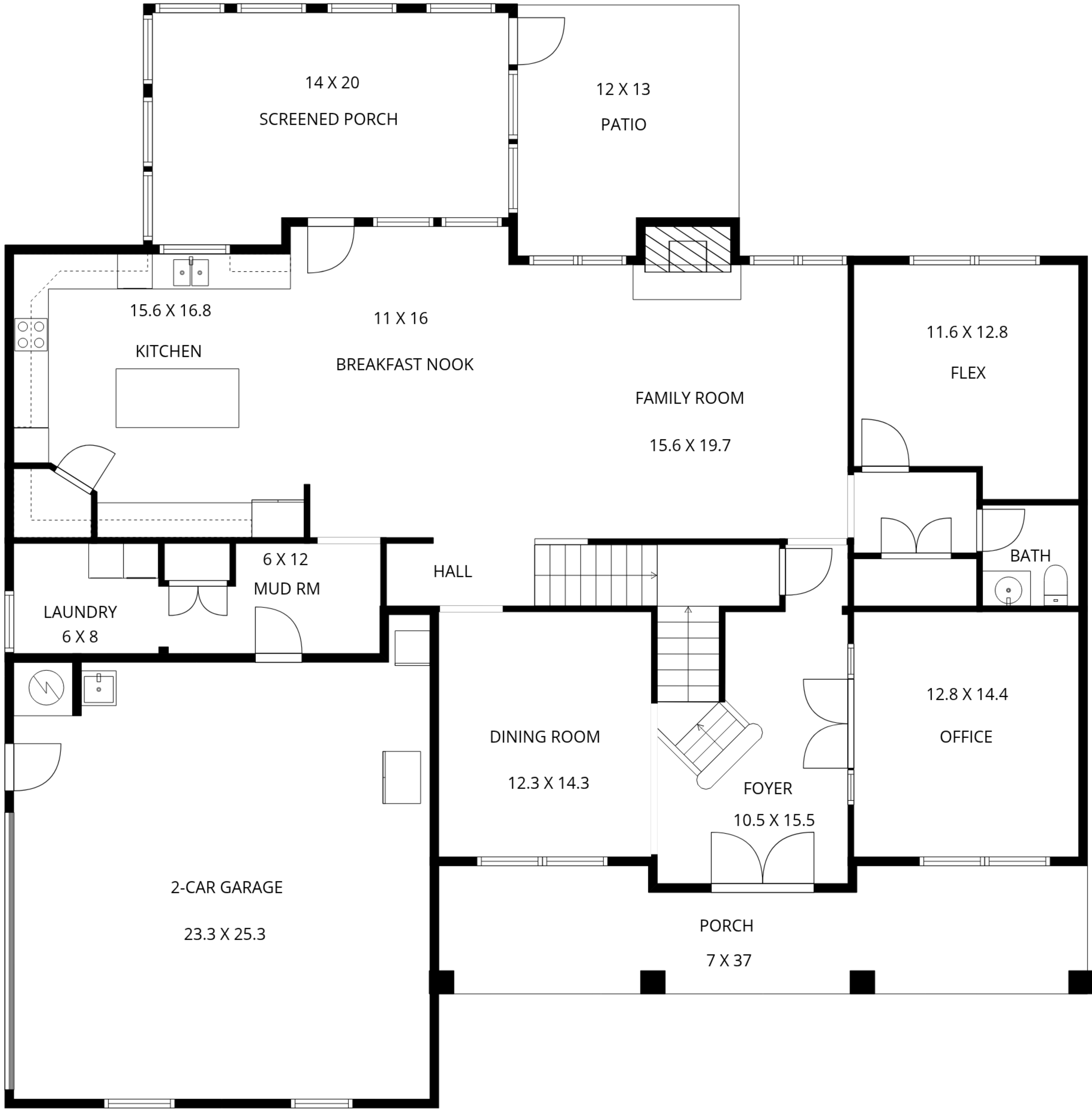
1ST FLOOR
