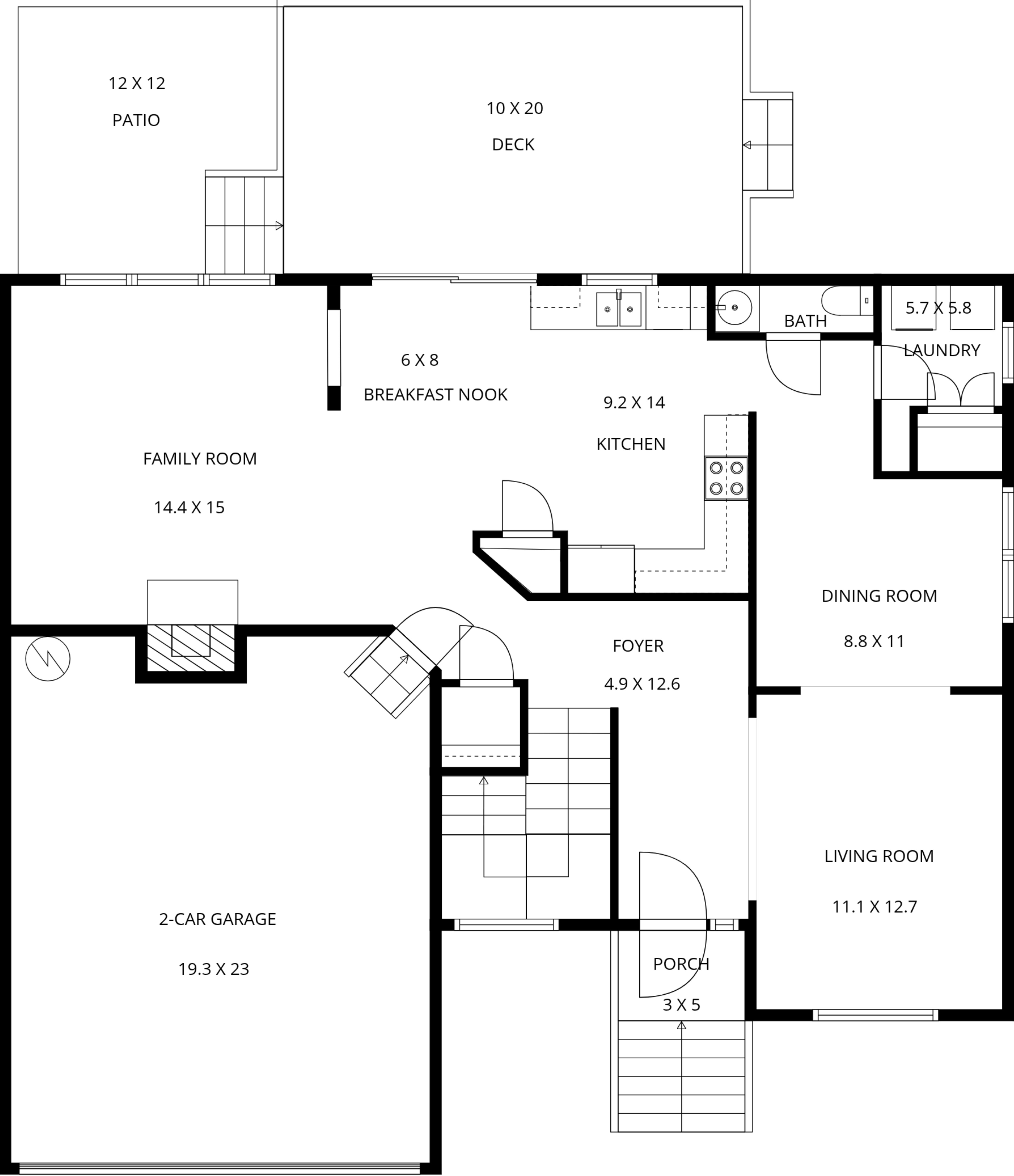
1ST FLOOR
