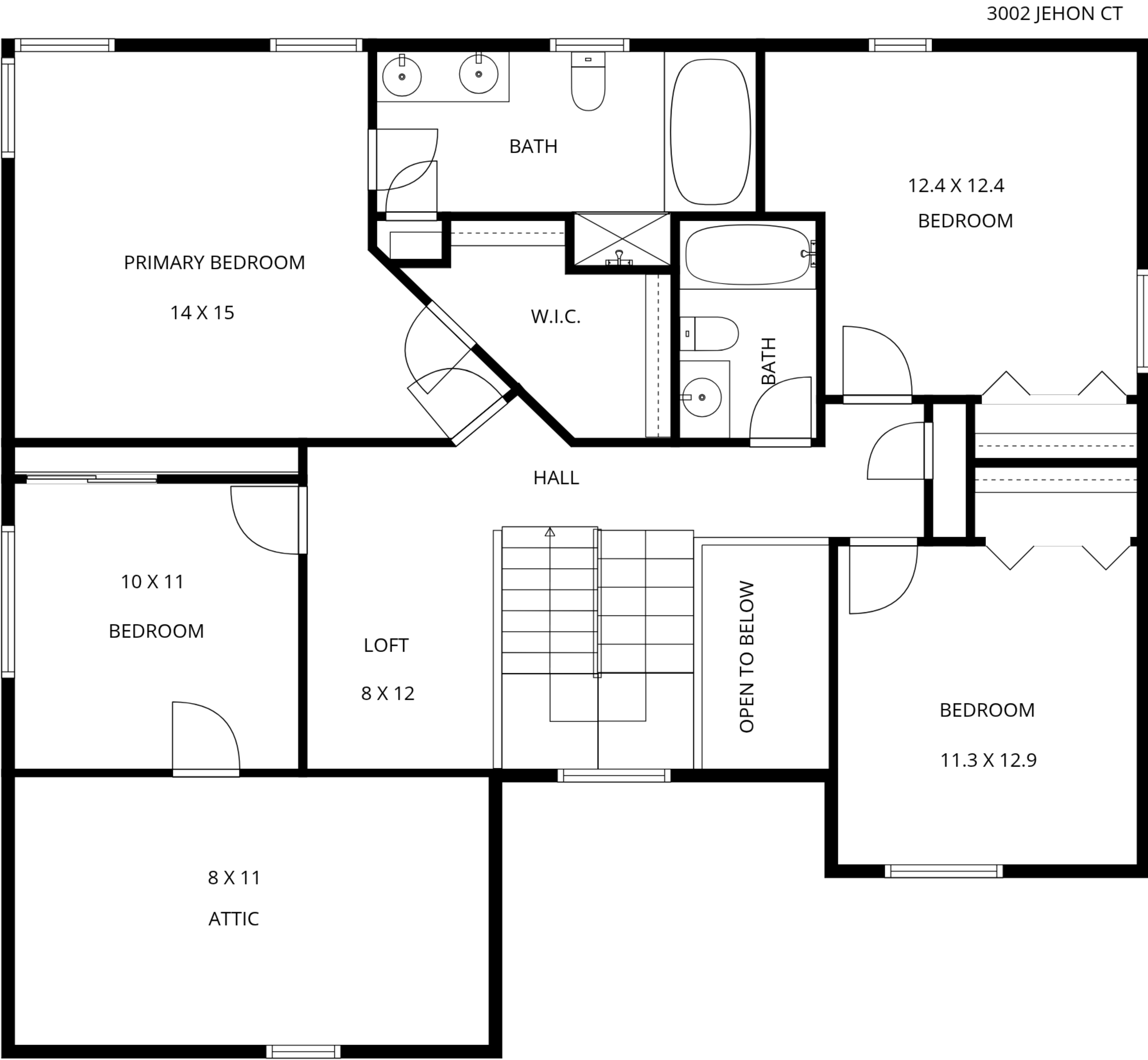
2ND FLOOR
