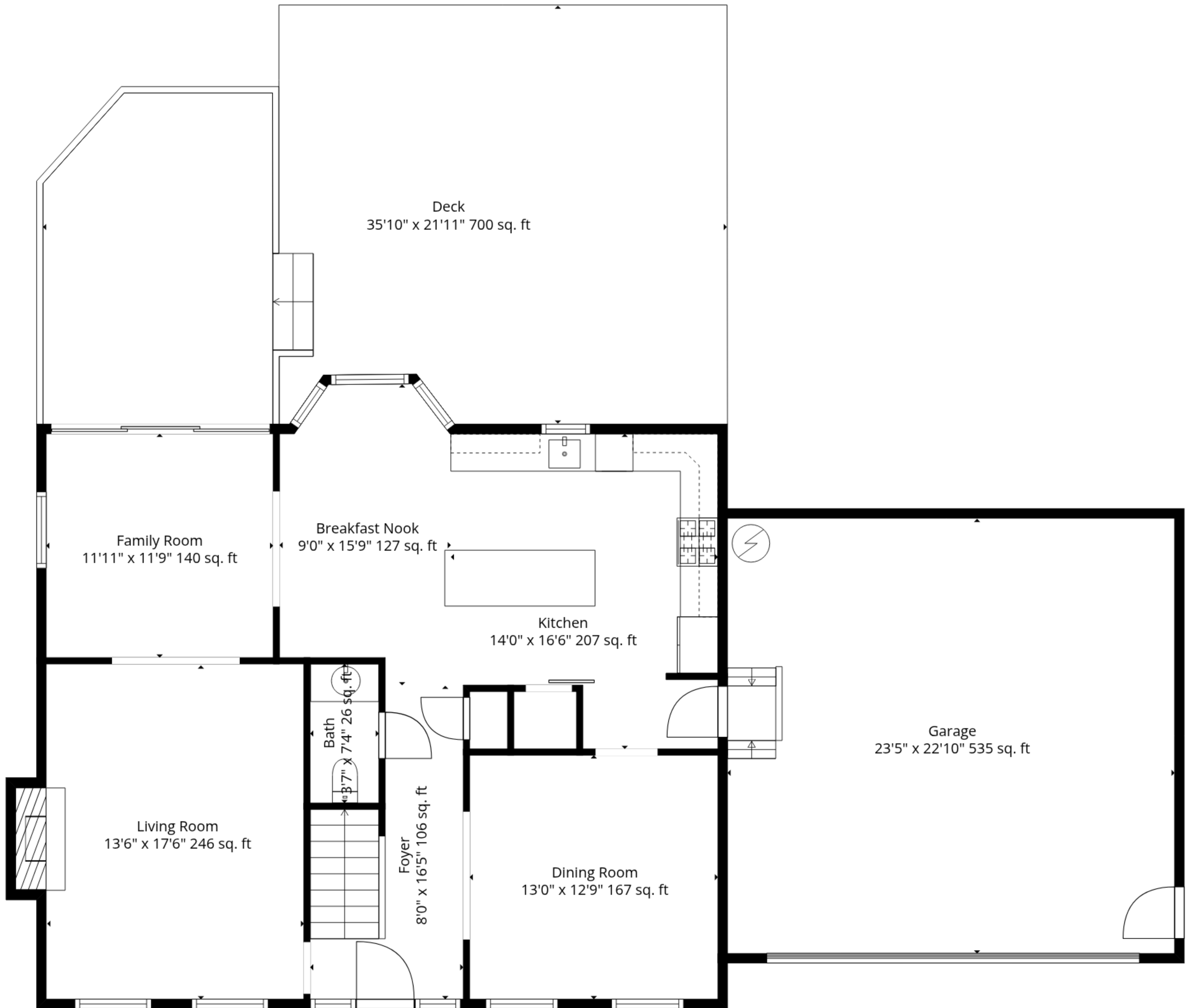
1st Floor
