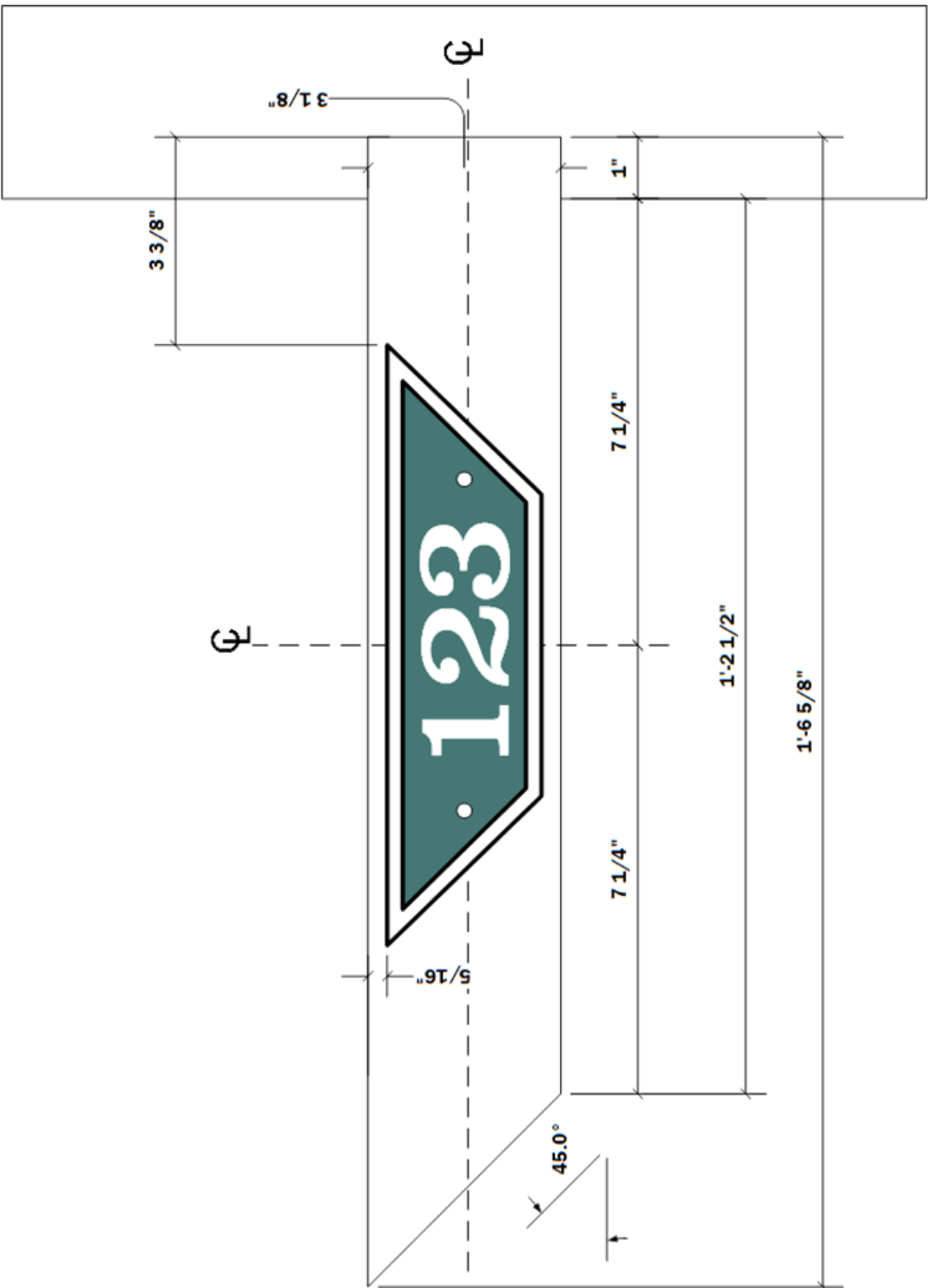
Figure C - West Park Mailbox Standard - Horizontal Cross-Member Detail and Dimensions
