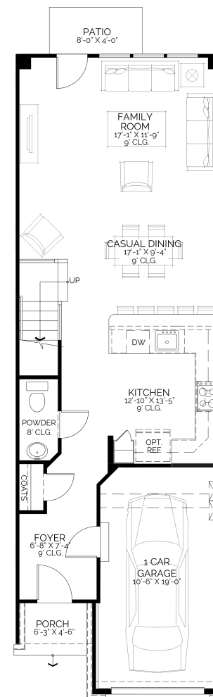
MAIN FLOOR
