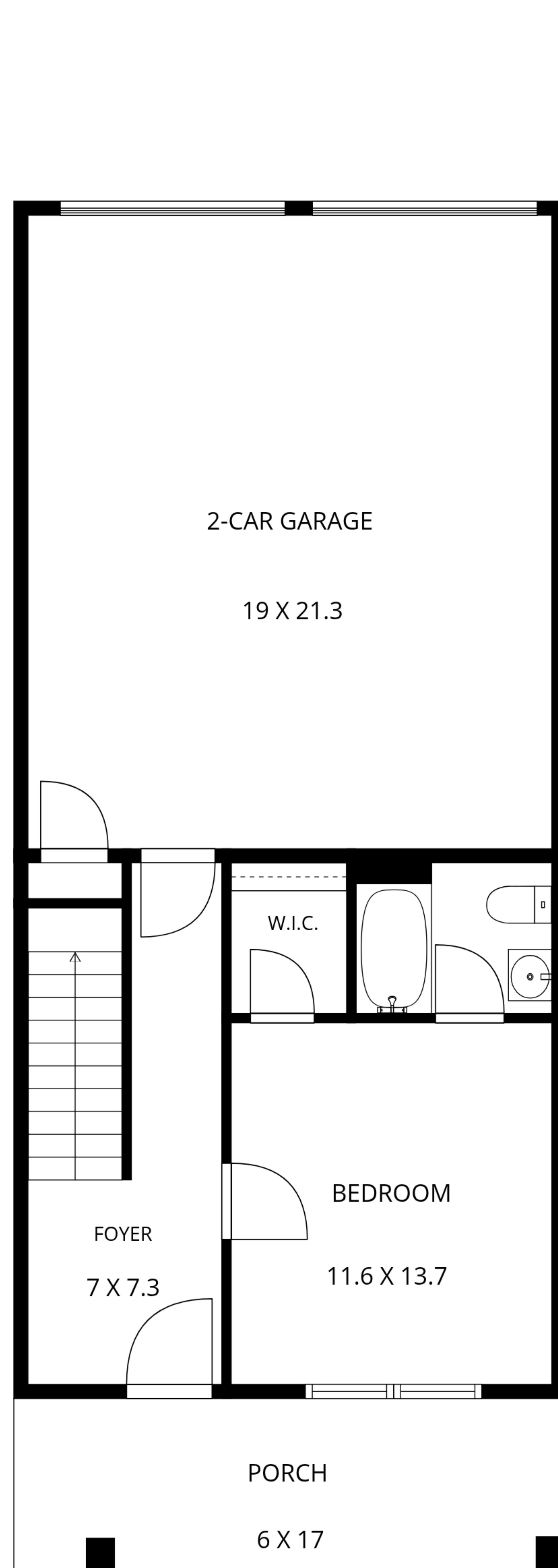
1ST FLOOR
