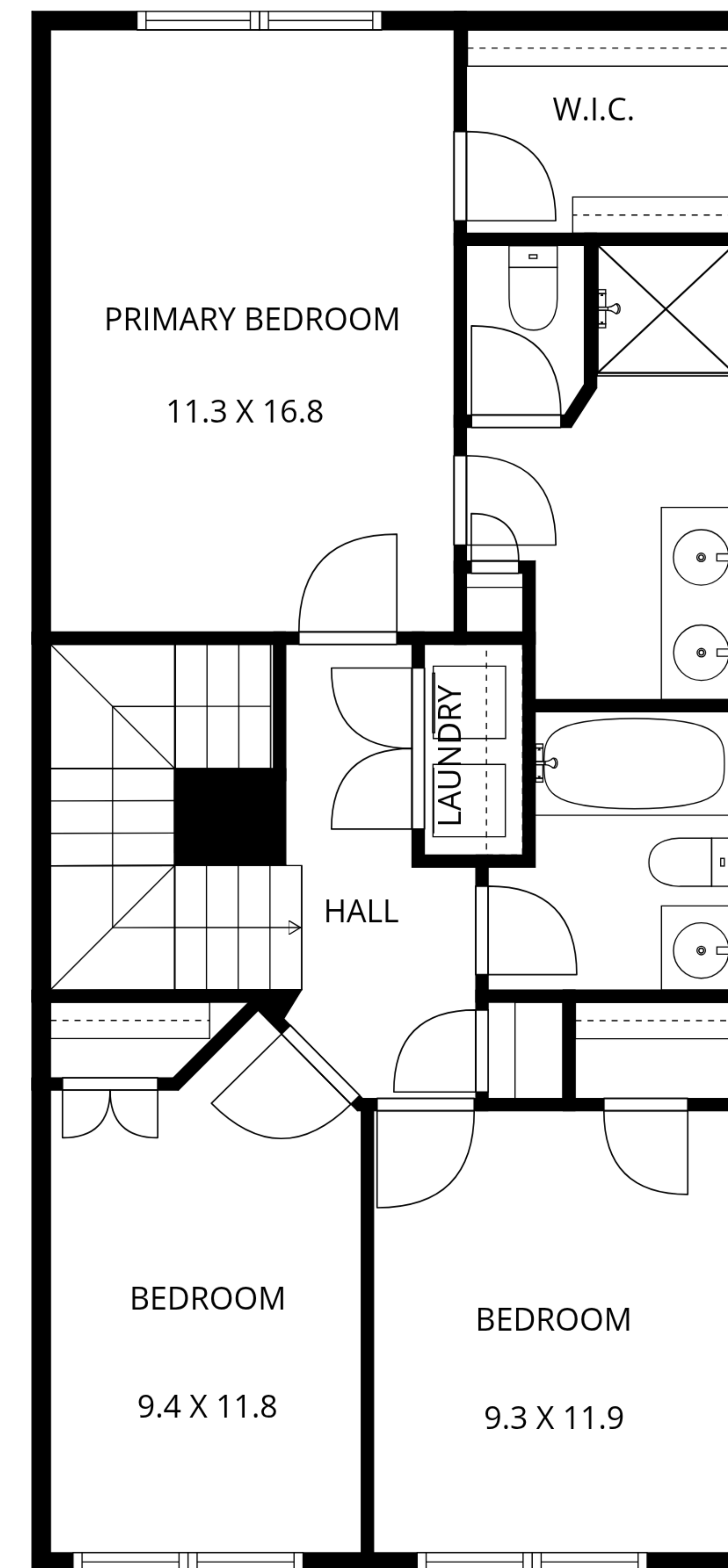
3RD FLOOR
