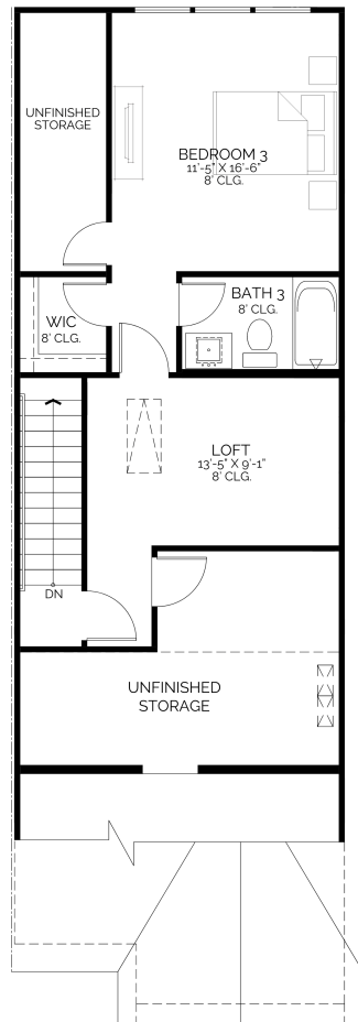
THIRD FLOOR
