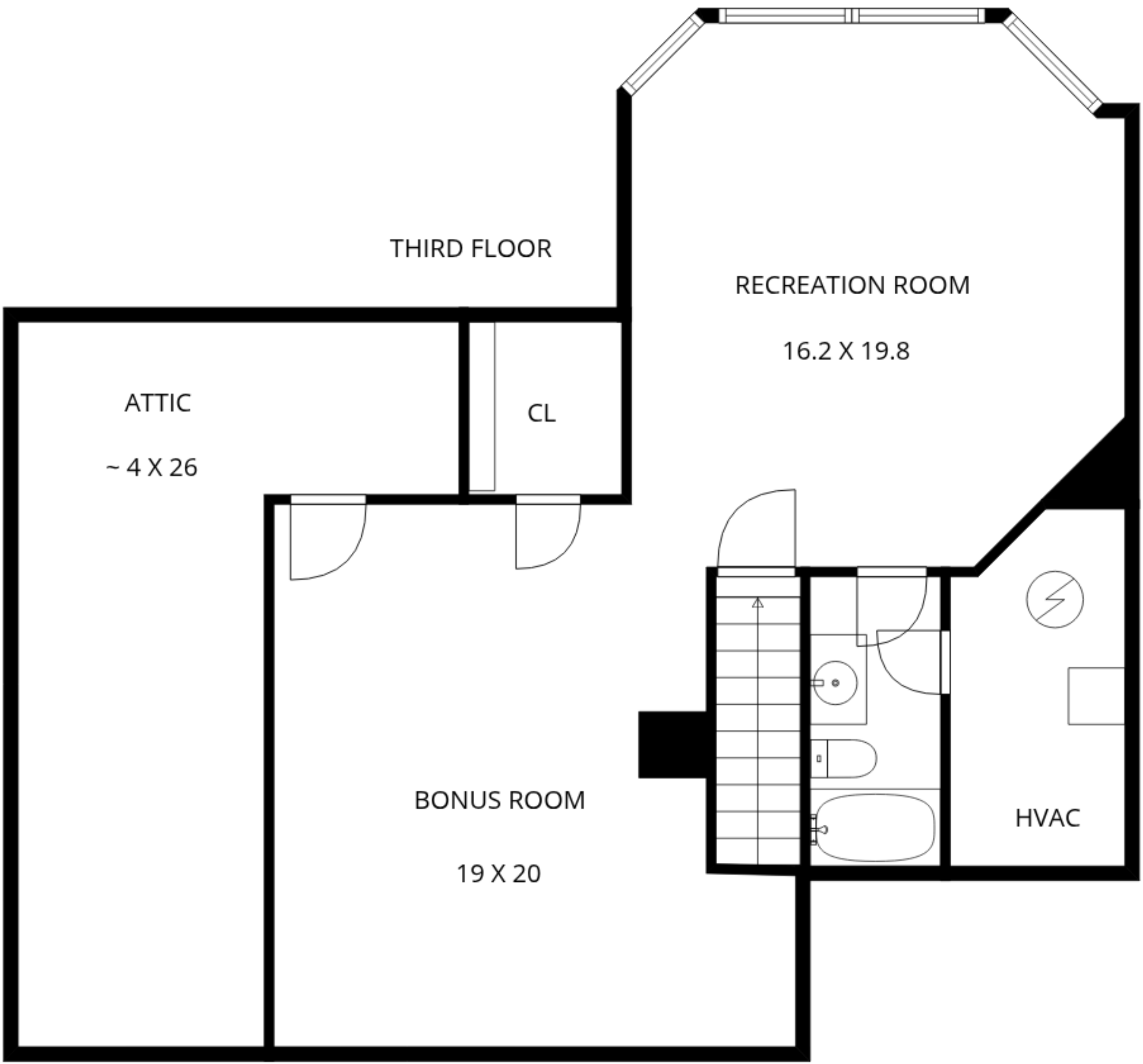
3RD FLOOR
