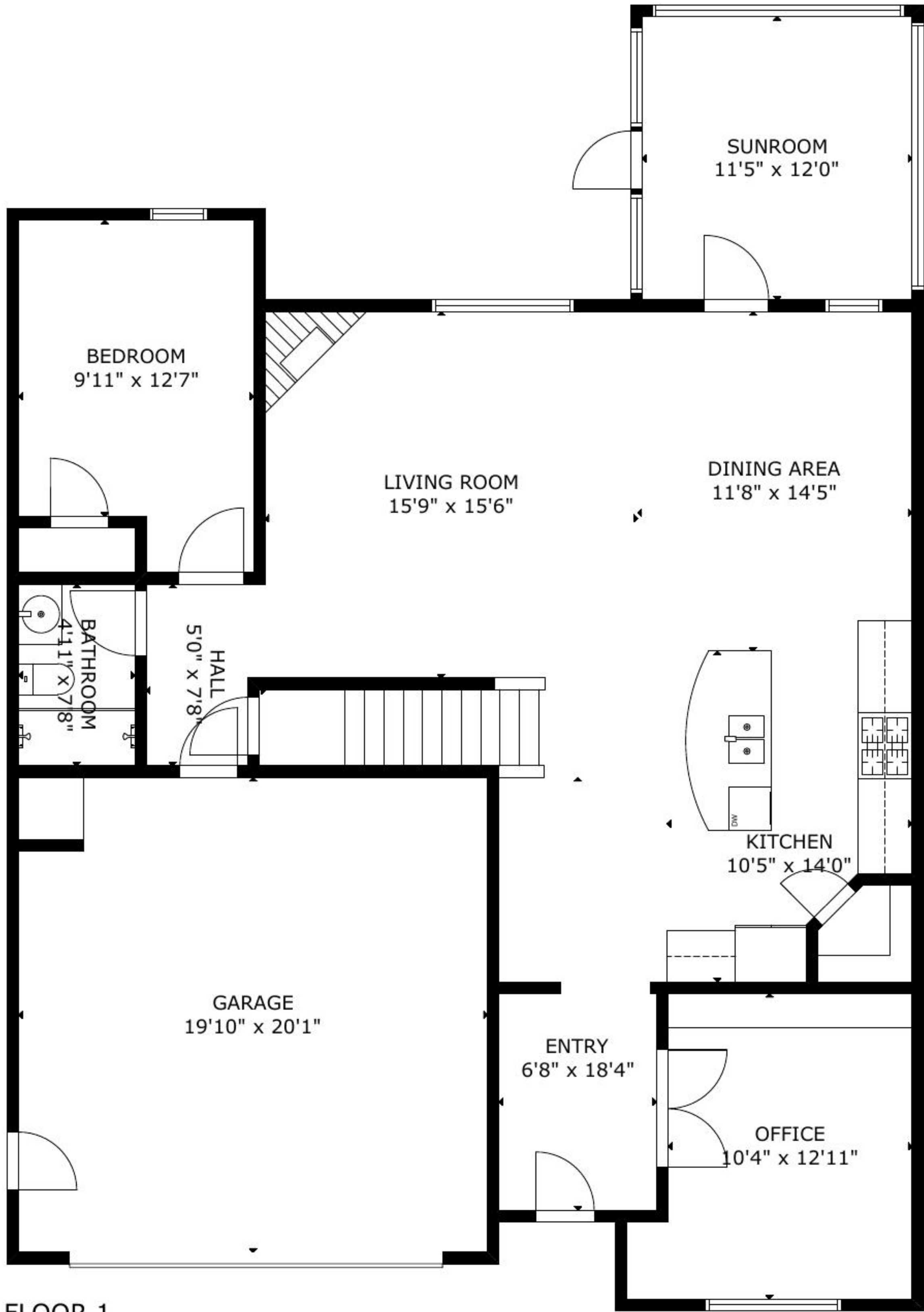
FLOOR 1
