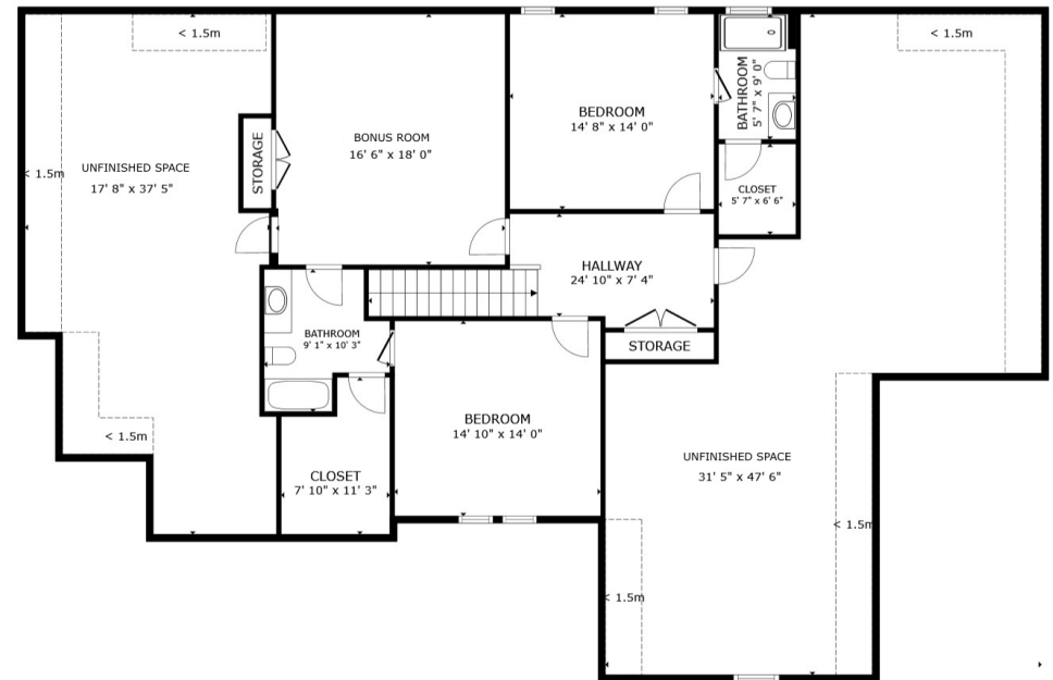
FLOOR 2 1,181 SQ.FT.
