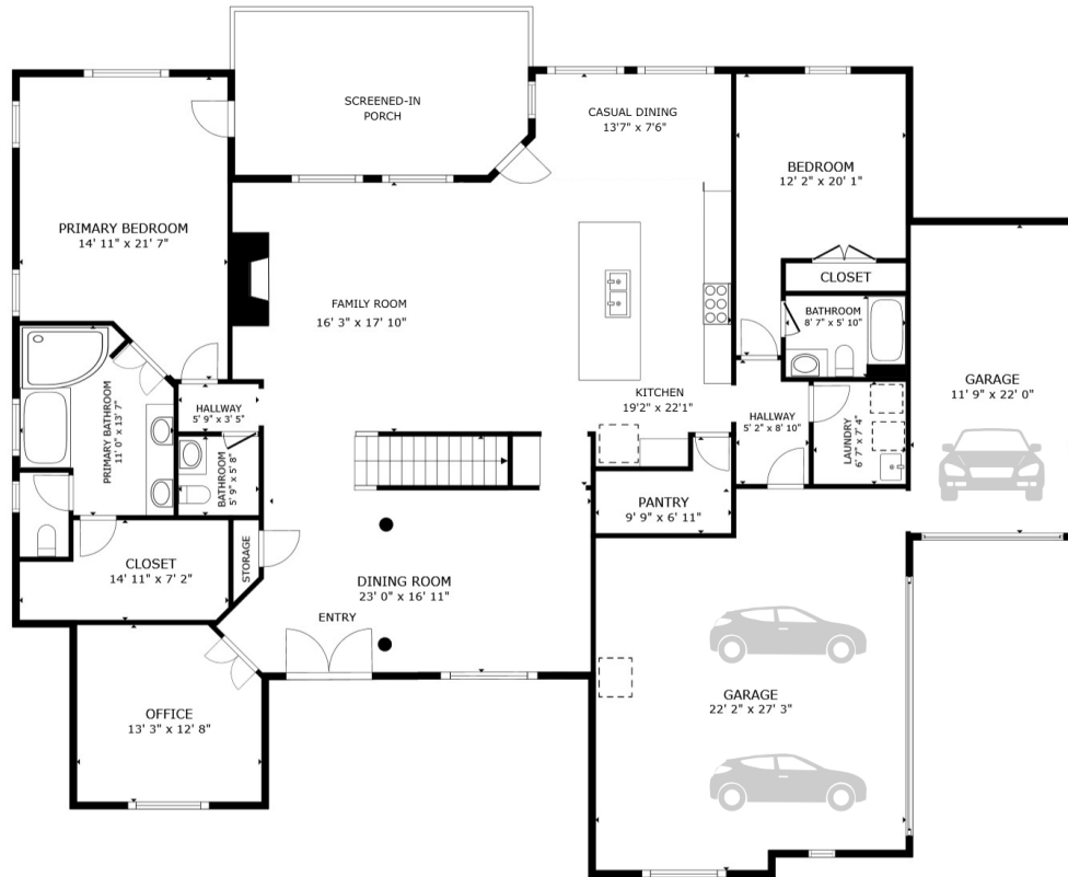
FLOOR 1 2,520 SQ.FT.
