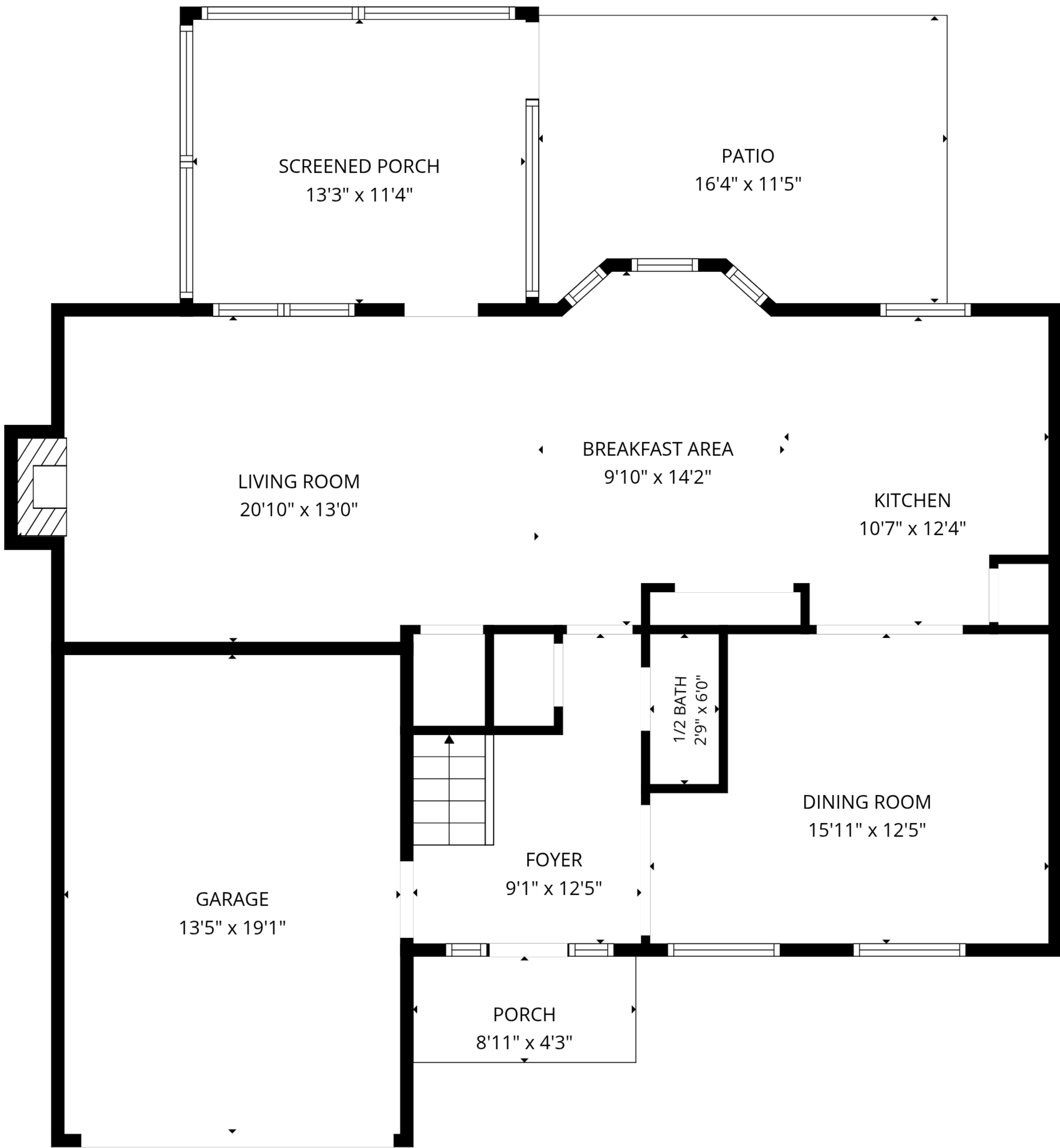
1st floor
